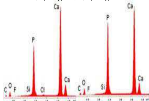
Pic.4. EDS-spectra of the coatings made from a) target 1, b) target 2
