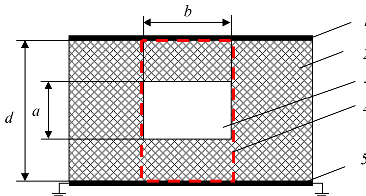
Fig. 1. Defective cable insulation model with “air pocket” defect: 1 is an electrode (plate of capacitor); 2 is a dielectric; 3 is “air pocket” (defect); 4 is the border of the defective insulation area 5 is a core (capacitor plate)
