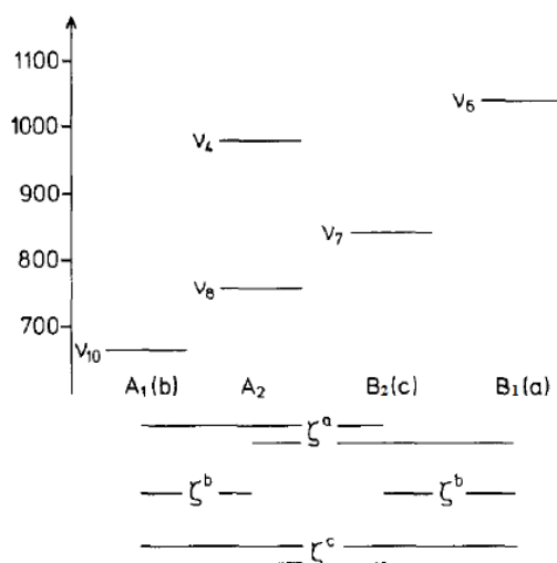
Fig. 1- The vibrational levels of cis-ethylene below 1100 \text{cm}^{-1} . At the bottom of the figure the symmetry of the levels are given together with their infrared band type. Possible Coriolis resonances around the a-, b-, and c-axes of the molecule are also included.
