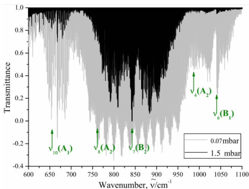
Fig.2 Overview spectra of the \text{C}_2\text{H}_2\text{D}_2\text{-cis} molecule in the region of 600-1100 \text{cm}^{-1}
