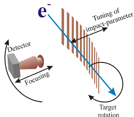
Figure 9. Scheme of CSPR focusing using a parabolic grating
