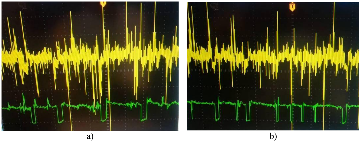
Fig. 2. Oscillograms of electric current and voltage: a) traditional one-jet gas shielding; b) double-jet gas shielding
