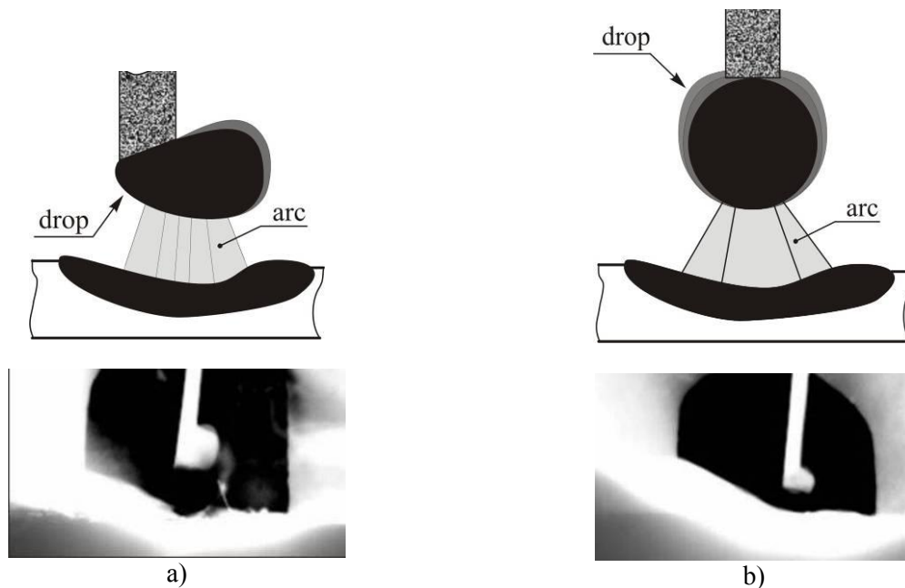
Figure. 1. The impact force of shielding gas jet on the drop: a) traditional one-jet gas shielding; b) two-jet gas shielding
