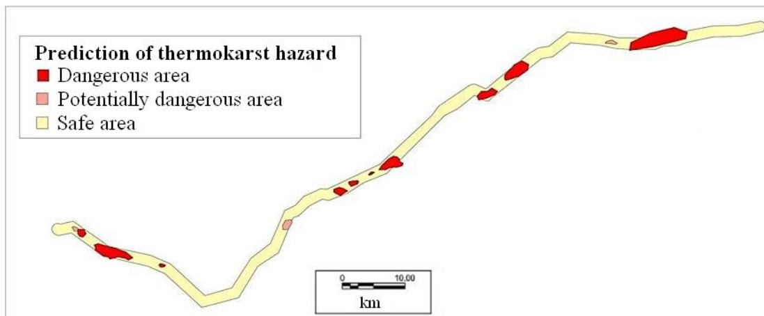
Figure 4. Zoning according to Thermokarst Hazard Ranking
