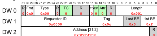
Рис. 1. Read Request TLP
