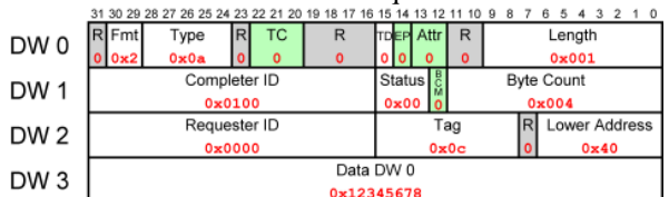
Рис. 2. Completion TLP
