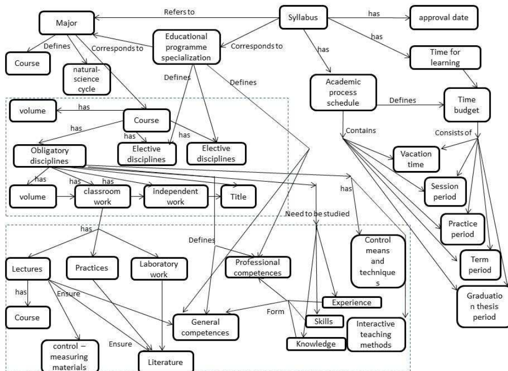
Figure 2.Academic subject ontology.
