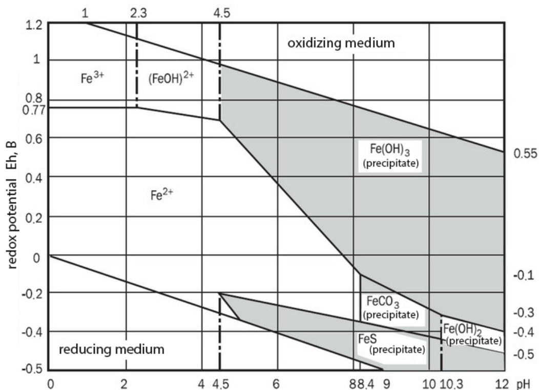
Figure 1. The possible reactions for the Fe-H 2 O system.
