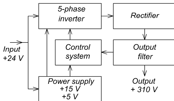
Figure 1. The block diagram of the device.
