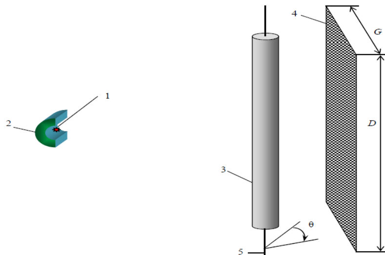
Figure 1. Continuous (discrete) rotation with the formation of two-dimensional projections: 1 – radiation source; 2 – source radiation protection; 3 – Object of inspection (OI); 4 – detector panel (matrix); 5 – axis of rotation of OI
