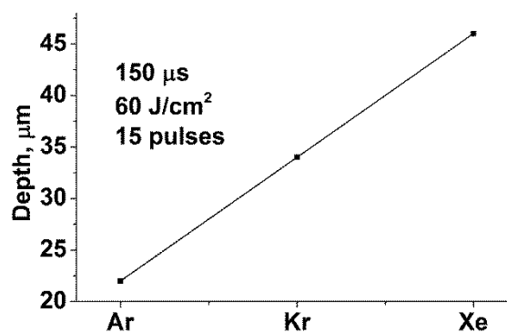
Figure 6. Dependence of the depth of modified surface layer on the type of plasma gas
