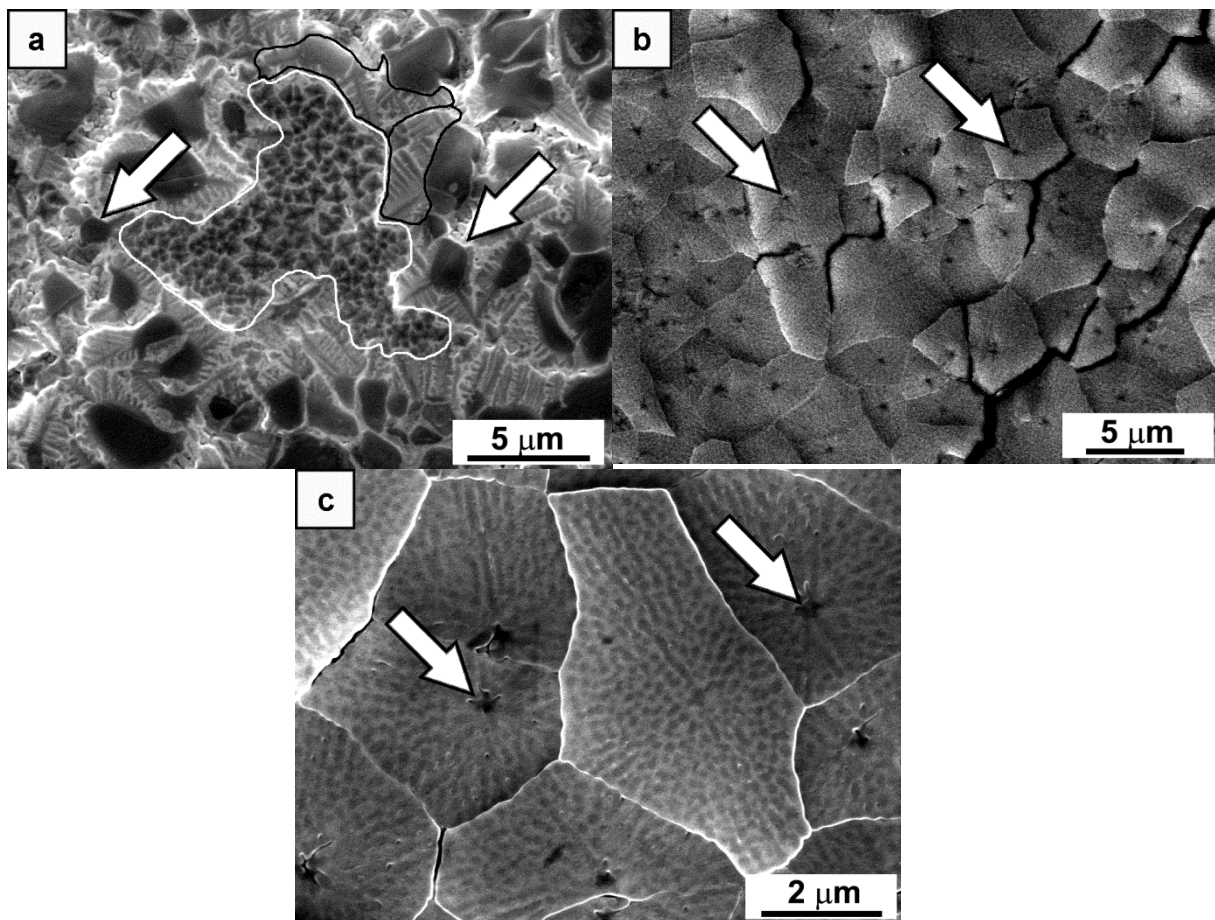
Figure 3. SEM images of the structure of the composite surface after pulse electron irradiation in the plasmas of argon (a), krypton (b) and xenon (c) ( 40 \text{ J/cm}^2 , 150 \mu\text{s} , 15 pulses)
