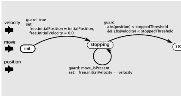
Fig 2. A CPS model inside
