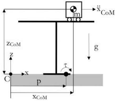
Рис. 3. Cart-Table Model
