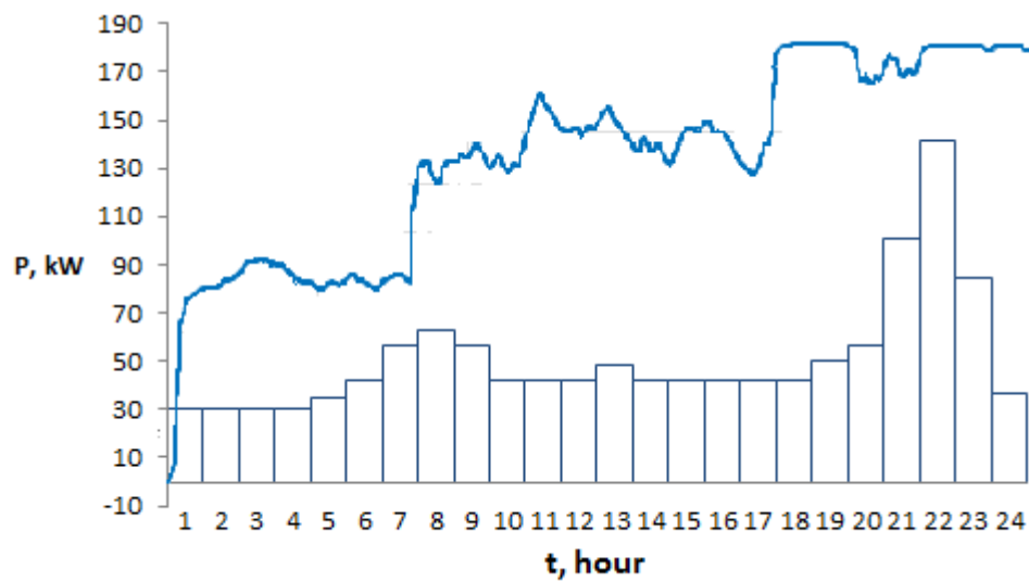
Figure 26 – Load coverage in the hottest day by wind turbines
