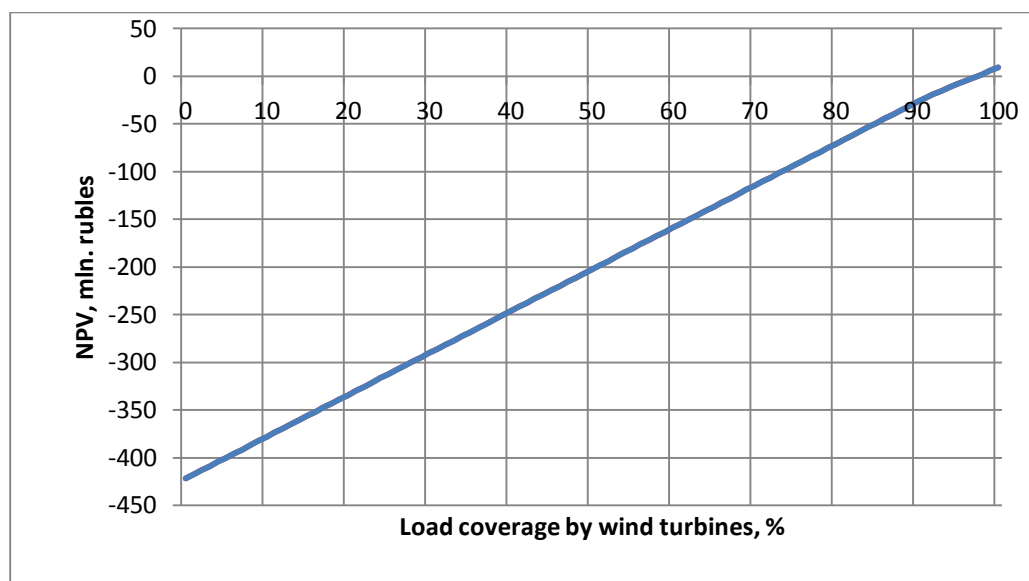
Figure 29 – Dependence of NPV on load coverage by wind turbines
