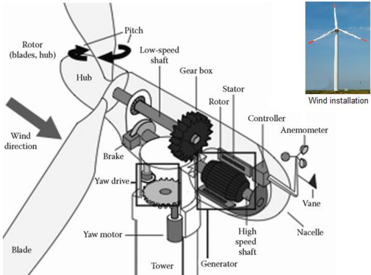
Figure 7 – Scheme of wind turbine components [13]
