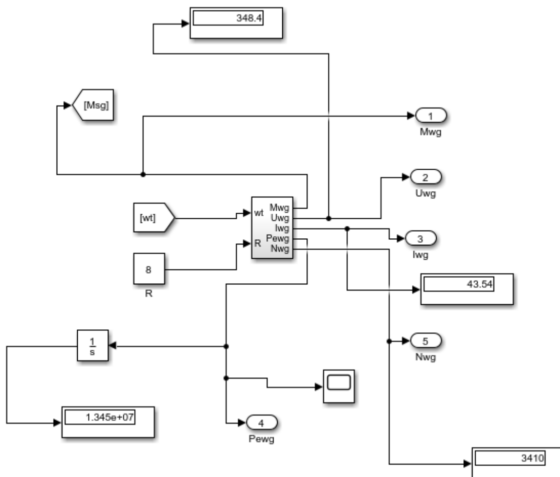
Figure 21 – Scheme of synchronous generator
