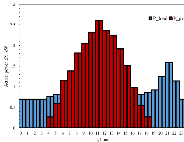
Figure 1. Daily dependencies of the generation of a photovoltaic plant in Russia and the total load of a rural house.
