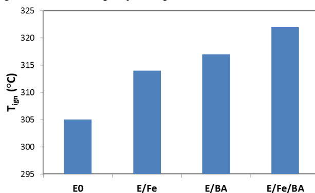
Figure 5. Ignition temperature of epoxy composites.
