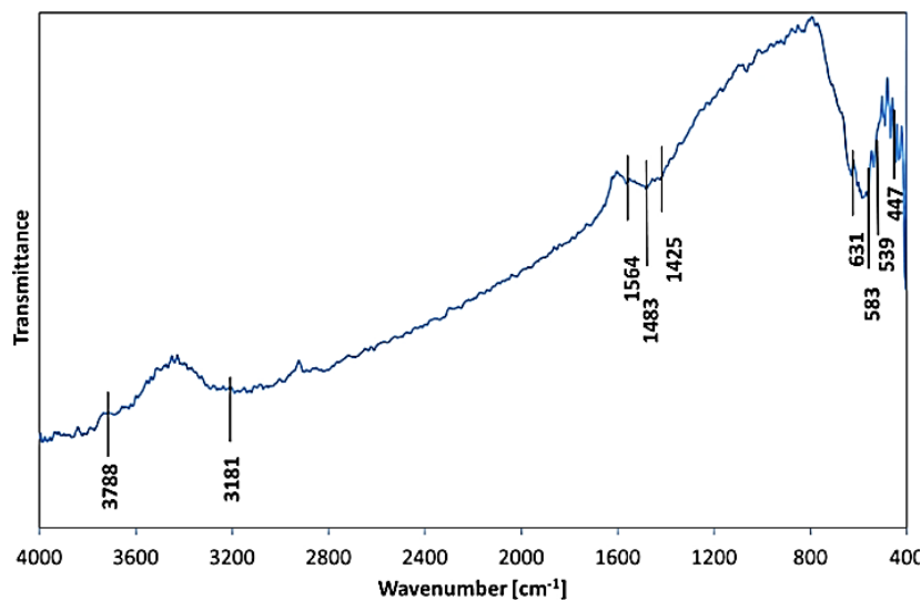
Figure 4. FTIR spectrum of Fe NP.
