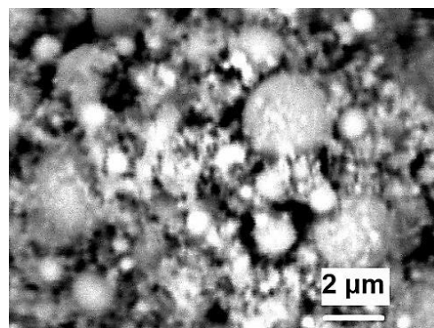
Figure 3. SEM image of Fe NP.
