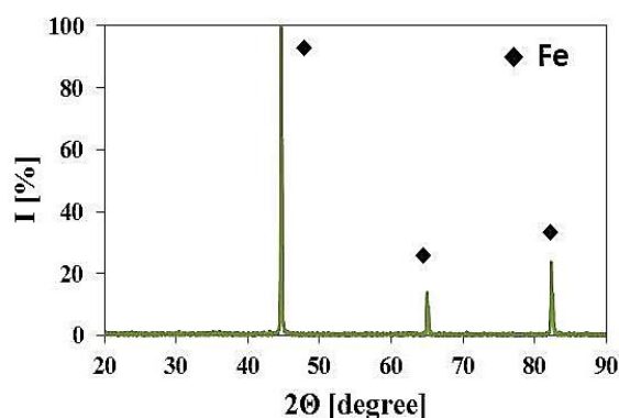
Figure 2. X-ray diffraction pattern of Fe NP.
