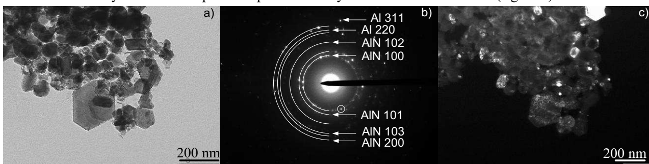
Fig. 1. TEM-images of synthesized product: a) bright-field image; b) SAED; c) dark-field image
