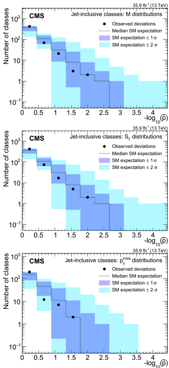
Fig. 13 Distribution of \tilde{p} values for the RoI scan in jet-inclusive classes for the M (upper), S_T (middle), and p_T^{\text{miss}} (lower) distributions
