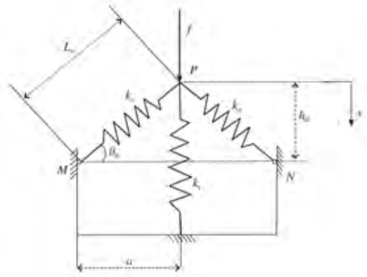
Fig. 1. Schematic representation of quasi-zero stiffness isolator
