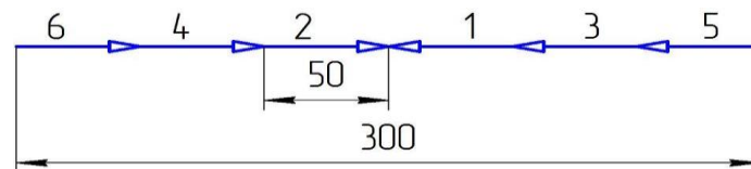
Figure 3. The scheme of welding seams.
