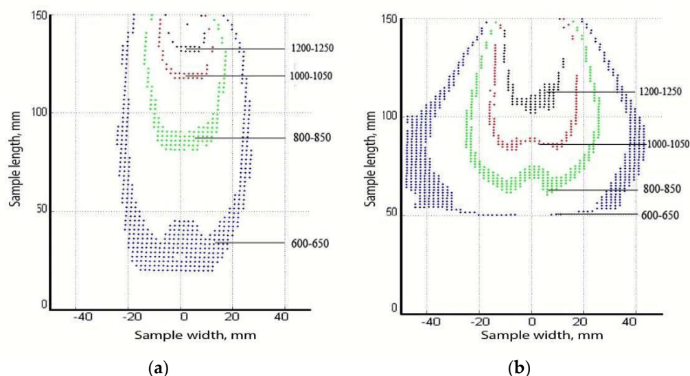
Figure 10. Patterns of temperature fields on the surface of the product welded by MMAW (electrodes LB-52U, diameter 3.2 mm), mode parameters I_w = 100 + 3A , U_w = 22 + 0.6 V , V_w = 13...14 cm/min: (a). inverter rectifier; (b). diode rectifier.
