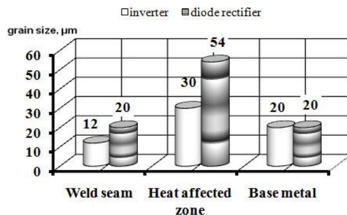
Figure 18. Average grain size in different zones of the weld as a function of the dynamic properties of the power source.
