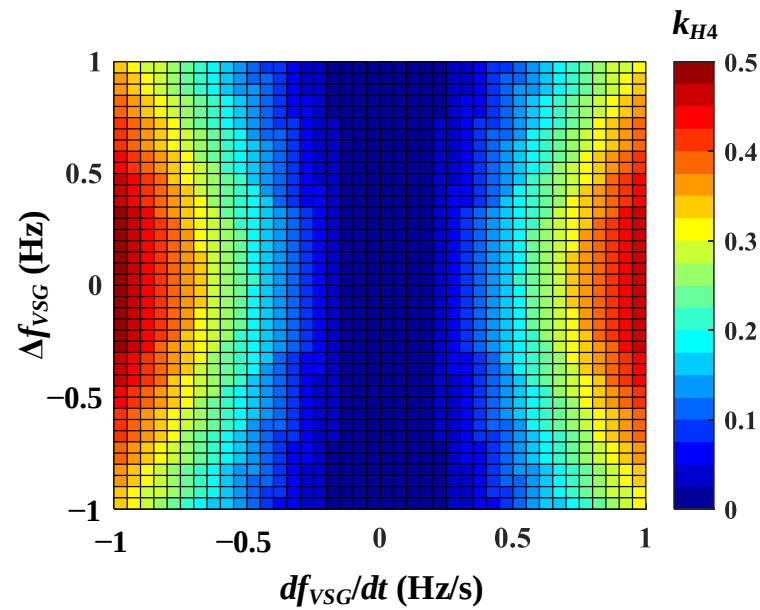
Figure 17. Variable k_{H4} coefficient.
