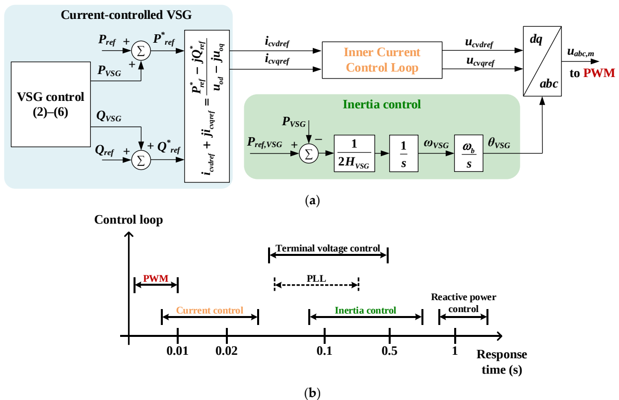
Figure 4. (a) Structural diagram of the CC-VSG and (b) control loops' time scale.
