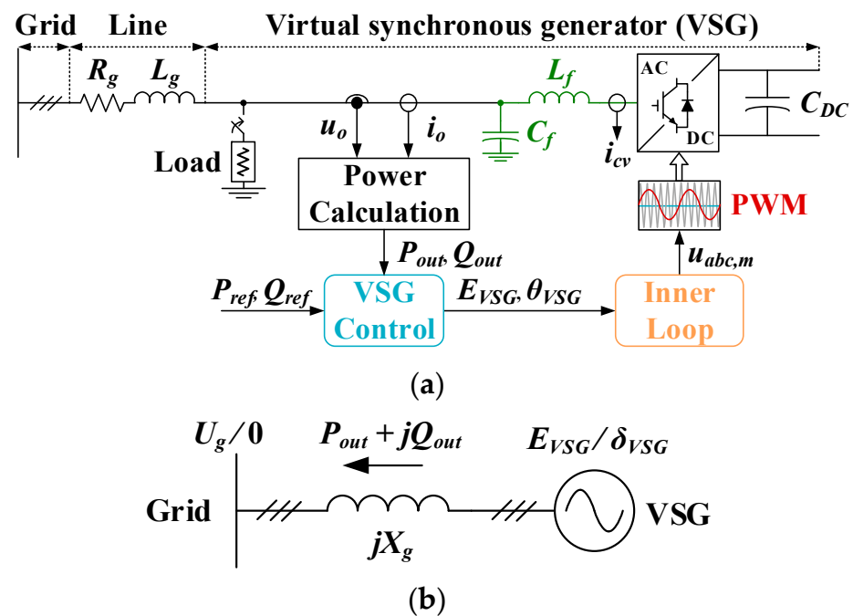
Figure 1. Test electrical network: (a) general diagram and control system structure; (b) simplified representation.
