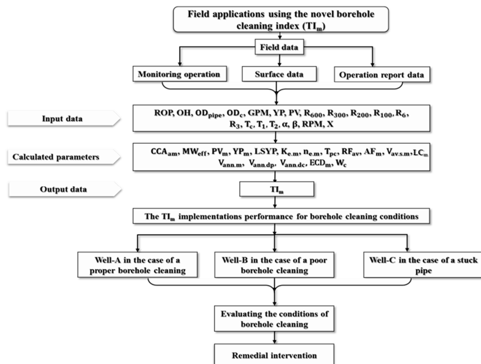
Figure 10. Flowchart to estimate the novel TI_m model in real time.
