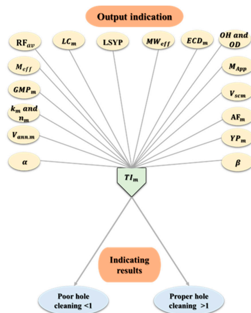
Figure 7. The measured, calculated, and output of the novel model TI_m , which is a real-time automated assessment for evaluating borehole cleaning conditions.
