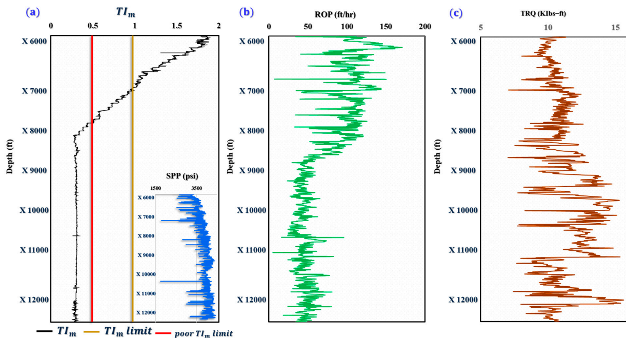
Figure 13. Application of TI_m in Well C in the case of a stuck pipe: (a) Well-C with poor borehole cleaning, (b) ROP, and (c) TRQ.
