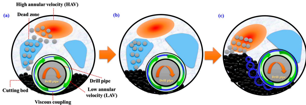
Figure 3. Influence of rotation on cuttings bed; (a) low RPM; (b) medium RPM; (c) at 120 RPM.
