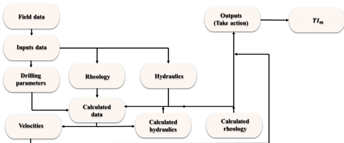
Figure 14. The automated process of using field data to evaluate the status of hole cleaning using TI_m for optimizing the drilling performance efficiency.
