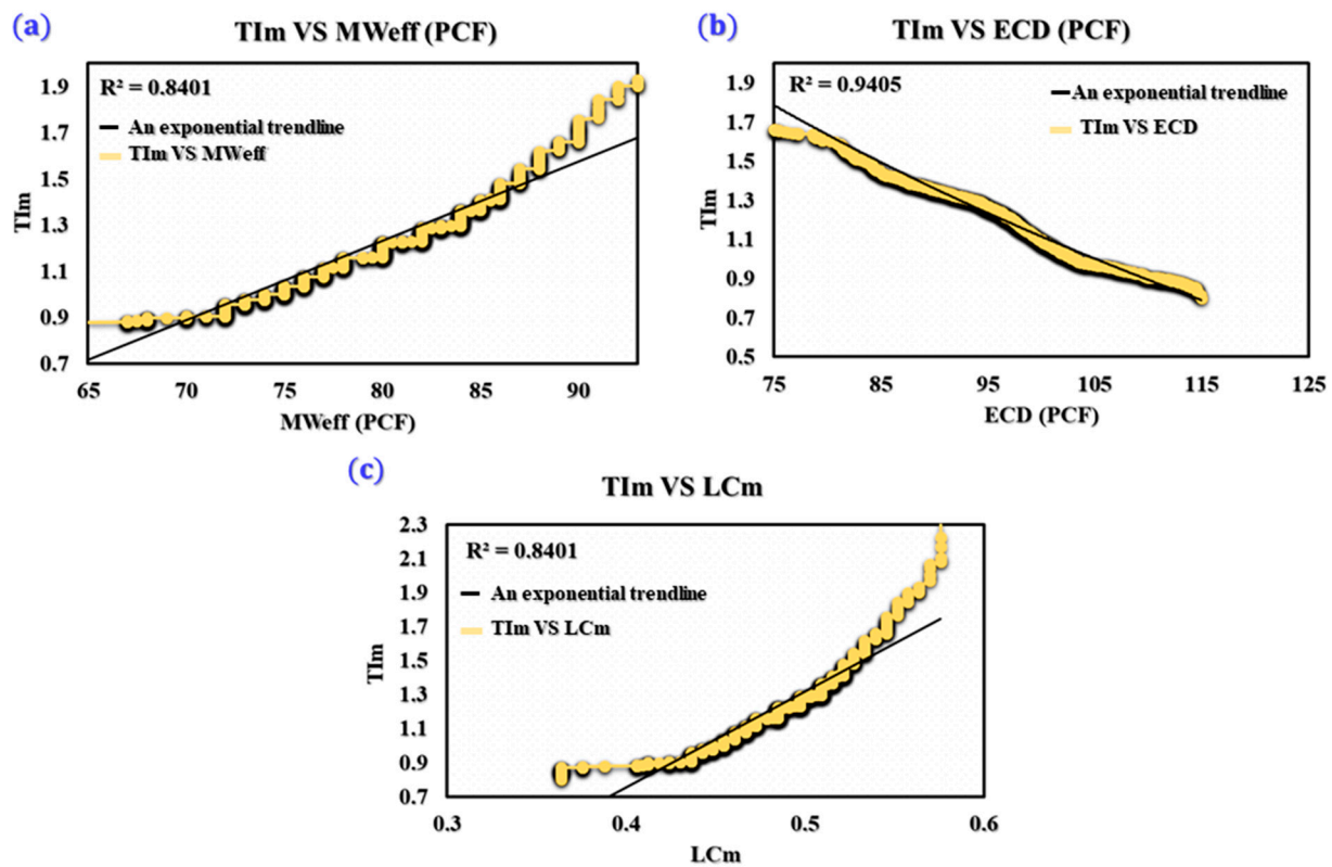
Figure 8. The performance of TI_m in relation to three key parameters: (a) MW_{eff} , (b) ECD, and (c) modified LC_m .
