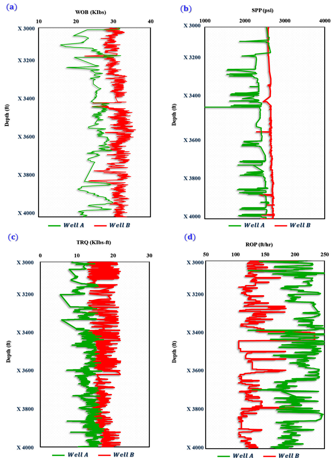
Figure 12. The changes in drilling parameters for Well-A with proper borehole cleaning and Well-B with poor borehole cleaning: (a) WOB, (b) SPP, (c) TRQ, and (d) ROP.
