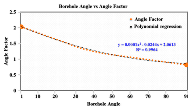
Figure 6. The interpolation of AF based on the borehole angle.
