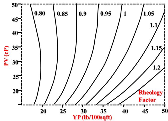
Figure 5. Graphical chart for the RF in borehole size 17–12''. Chart is based on Luo's chart [38].
