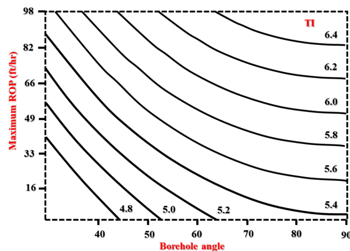
Figure 4. Read of maximum ROP based on the TI values and the borehole angle. Chart is based on Luo's chart [37].
