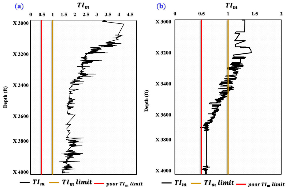
Figure 11. Application of TI_m in offshore Well-A with proper borehole cleaning (a) and Well-B with poor borehole cleaning (b).
