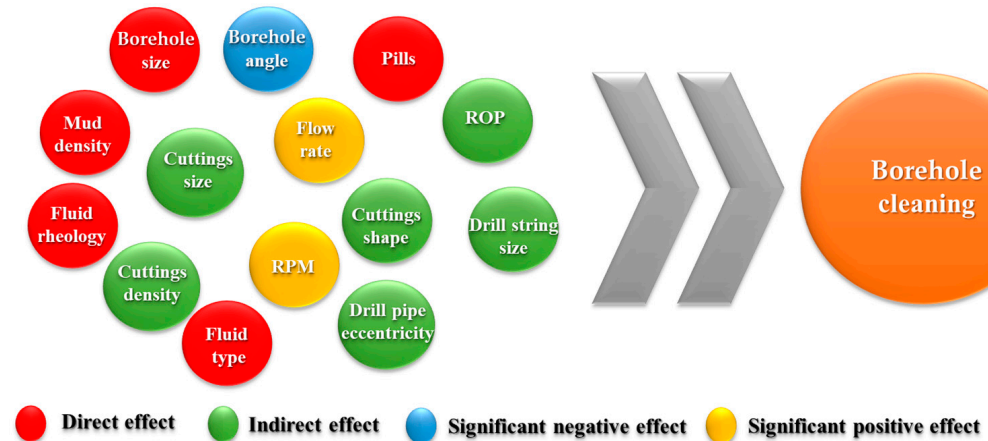
Figure 2. Parameters and their effect on borehole cleaning.
