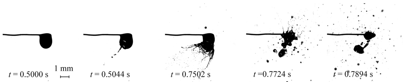
Figure 3. Puffing of water/rapeseed oil droplets ( R_{d0} \approx 1.3 mm, \eta_f \approx 80\% , T_a \approx 773 K).
