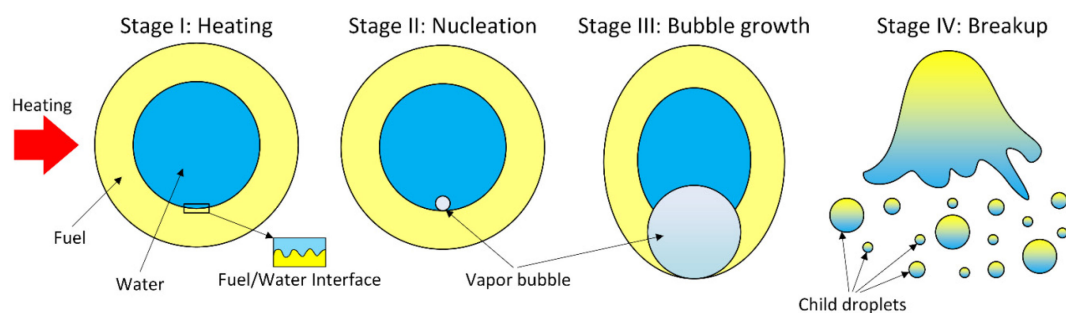
Figure 4. Physical model simulating the micro-explosive breakup of a two-liquid droplet into secondary fragments.
