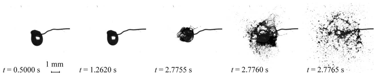
Figure 2. Micro-explosive breakup of water/kerosene droplets ( R_{d0} \approx 1.3 mm, \eta_f \approx 80\% , T_a \approx 773 K).
