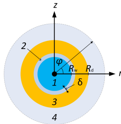
Figure 6. Schematic solution space (1—water; 2—water vapor; 3—fuel; 4—air); R_w is the water core radius; R_d is the droplet radius.
