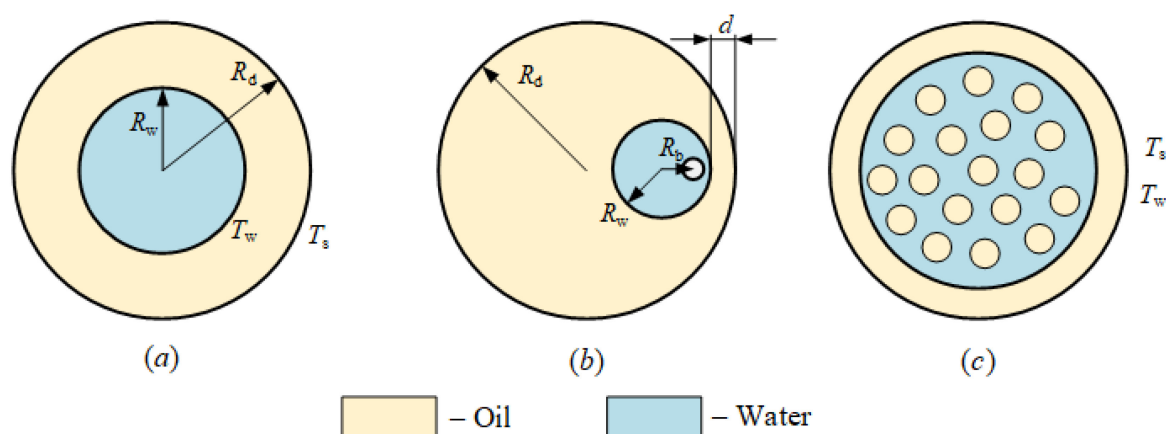
Figure 5. Typical schematics for describing micro-explosion: (a)—[27,38], water droplet of radius R_w inside a fuel droplet of radius R_d , T_w is the temperature at the water–fuel interface, T_s is the temperature at the droplet surface; (b)—[3], emulsion droplet geometry; (c)—[89], oil membrane forming in an emulsion droplet.
