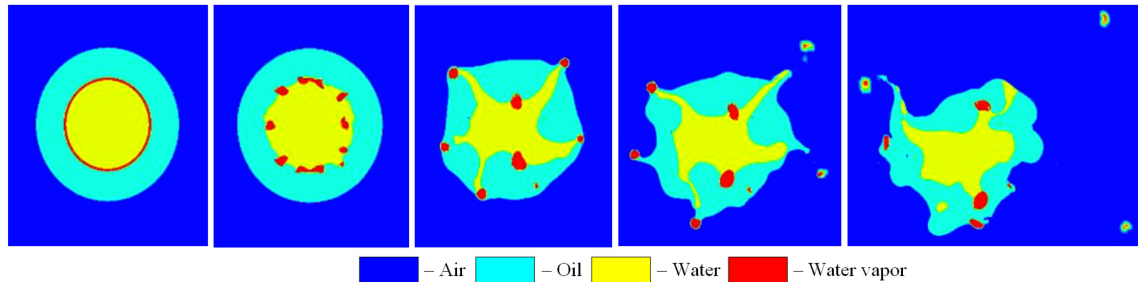
Figure 7. Typical outcomes of different-scale droplet fragmentation ( R_{d0} = 1.3 mm, R_{v0} = 0.8 mm, R_{w0} = 0.75 mm, water/rapeseed oil, combustible liquid concentration 80%, vapor layer thickness 0.05 mm, initial pressure in the vapor layer 10^6 Pa).
