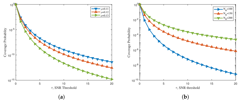
Figure 3. (a) Uplink coverage probability of the proposed mMTC network for various \rho values and (b) uplink coverage probability of the proposed mMTC network for various N_R values.
