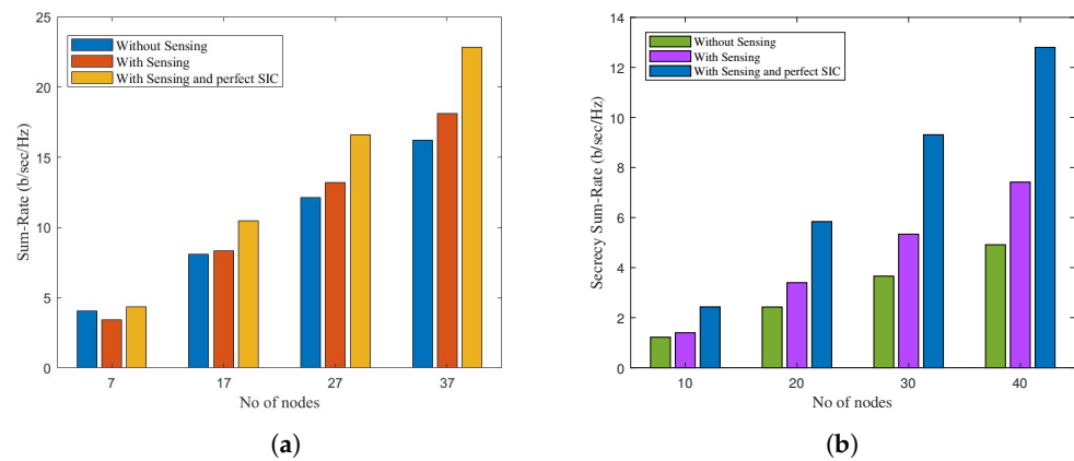
Figure 4. (a) Sum rate of the proposed NOMA-based mMTC network without Eve and (b) secrecy sum rate of the proposed NOMA-based mMTC network with Eve.
