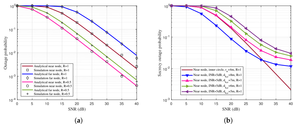
Figure 5. (a) Outage probability of downlink NOMA-based mMTC network and (b) secrecy outage probability of downlink NOMA-based mMTC network.
