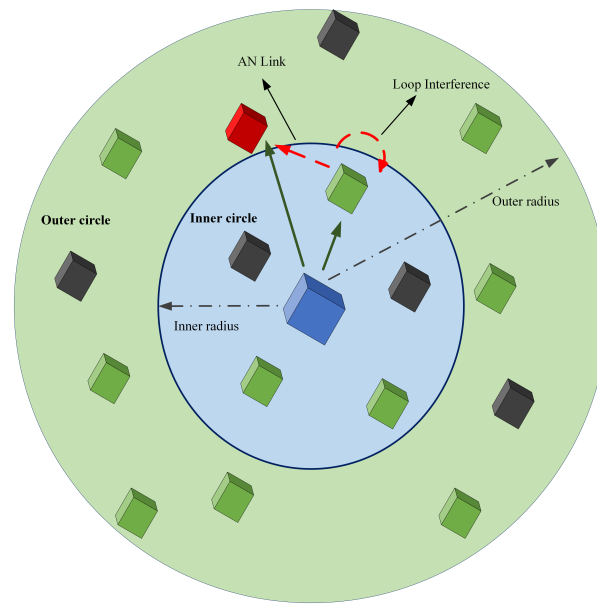
Figure 1. The proposed NOMA-assisted mMTC Wireless Networking System model, with active (green) and inactive (black) nodes distributed randomly in the circular region; an Eve node (red) tries to trace the confidential message information, and the blue node acts as the head node.
