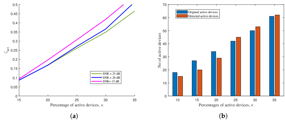
Figure 2. (a) Normalized average mean square error of active device detection and (b) active device detection of the proposed mMTC network.
