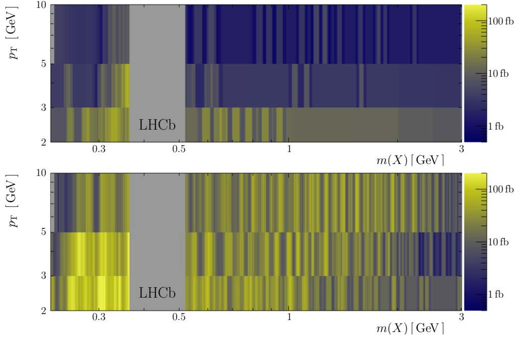
Figure 9. Upper limits at 90% confidence level on the cross section \sigma(X \rightarrow \mu^+\mu^-) for the (top) promptly produced and (bottom) inclusive searches for displaced X \rightarrow \mu^+\mu^- decays.
