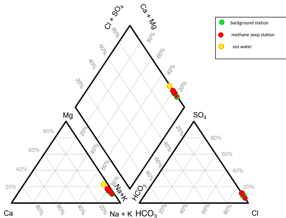
Figure 2. Piper-diagram of the studied pore-water. Green filled circles mark the pore-water sampling from background stations, red filled circles mark the pore-water sampling from methane seep stations.
