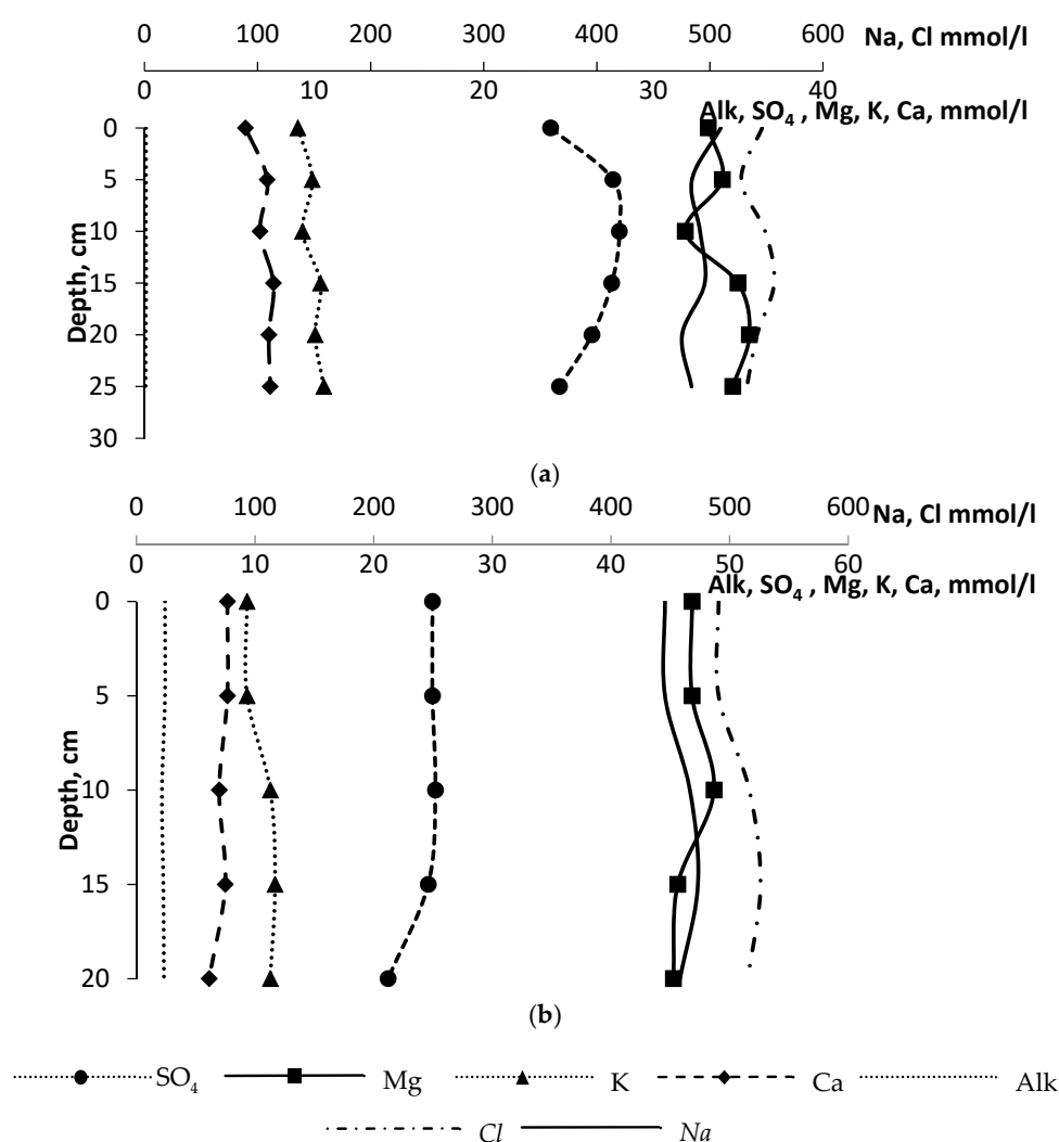
Figure 3. Concentration profiles: (a) background sites; (b) “methane seep” sites.
