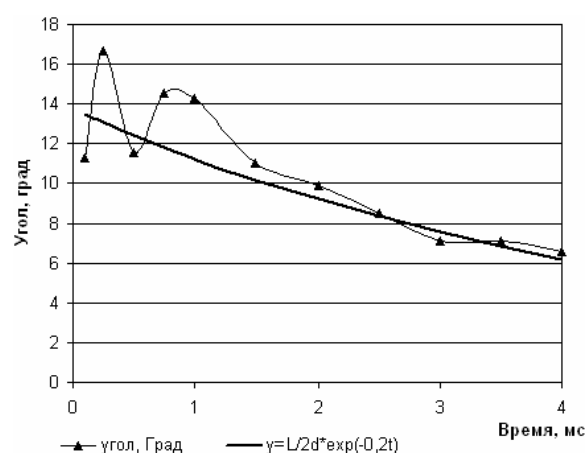
Fig. 6. Dependence of flow root angle on time of its development
