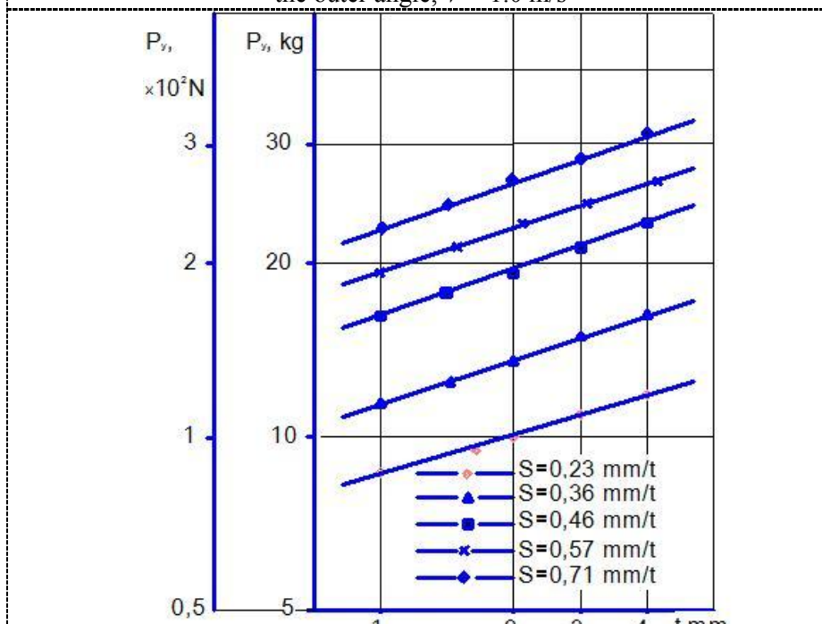
Figure 2b. The effect of the depth of cutting and supply on the component P_y , GI25-VK6, cutting tool – VAZ, three-faceted insert with the outer angle, V = 1.0 m/s
