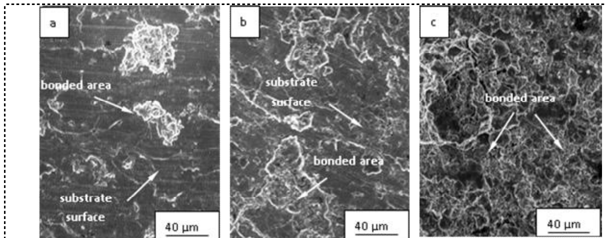
Figure 5. Surfaces, modified with ultrasonic tool, after failure of coatings a) nickel; b) chromium; c) molybdenum
