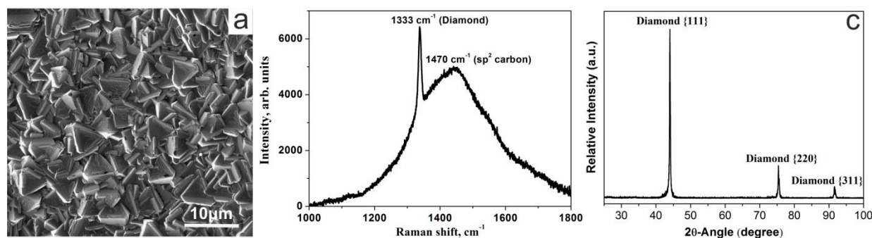
Figure 3. The data about structure and phase composition of obtained diamond coatings: SEM image of 25 μm film (a), Raman spectra (b) and x-ray diffraction pattern (c).
