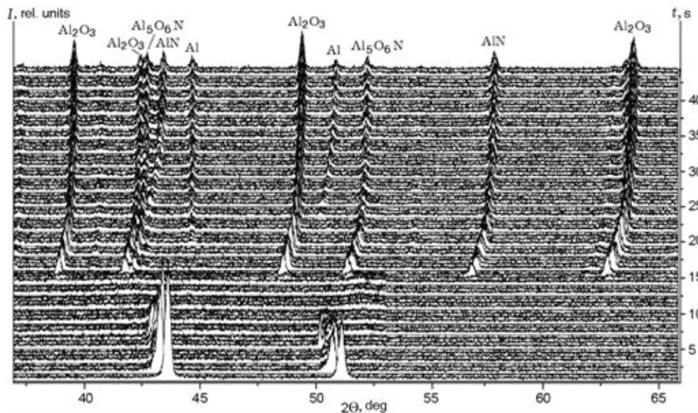
Fig. 2. Time scan of diffractograms of the burning compacted aluminum nanopowder (surface).
