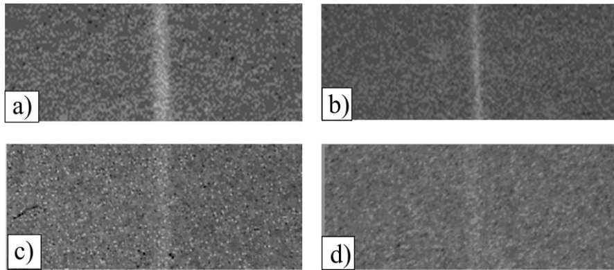
Figure 4. The foil images measured at the orientation of the Ta foil relative to the axis of radiation beam \theta_f = 0,6^\circ and 0^\circ , (a) and (b), respectively; (c) and (d) - at \theta_f = 0,6^\circ and with the steel plate-absorbers 20 and 55 mm thick, respectively. The images enlarged additionally for demonstration.
