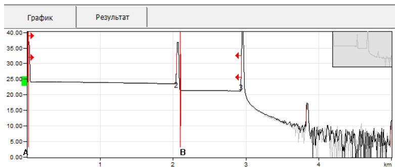
Figure 8. Reflectogram for the wavelength \lambda_1 = 1550 nm.
