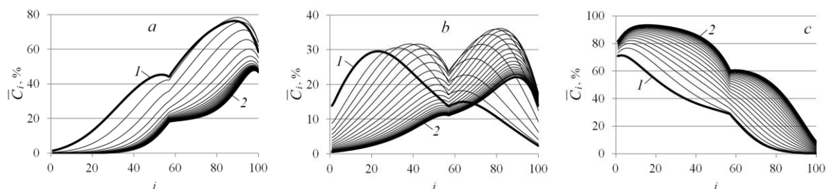
Figure 5. The change of the weighted average concentration of germanium isotopes in cascade stages during a nonstationary process: a – ^{72}\text{Ge} ; b – ^{73}\text{Ge} ; c – ^{74}\text{Ge} ; 1 – initial state; 2 – final state.
