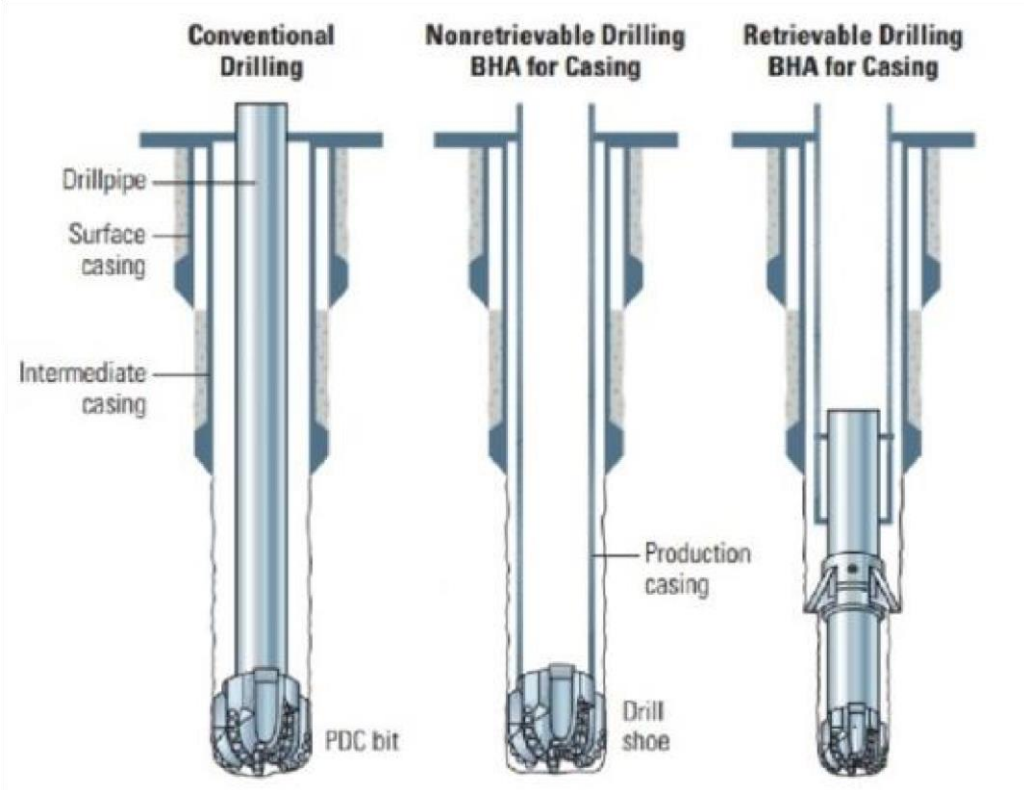
Figure1 _Conventional drilling and casing drilling BHAs
