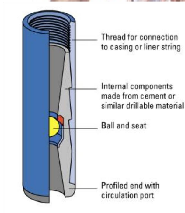
Figure 7 – Overdrive system
