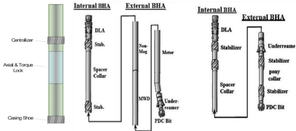
Figure 4 – Figure 5 Retrieval BHA for (a) directional drilling and (b)
