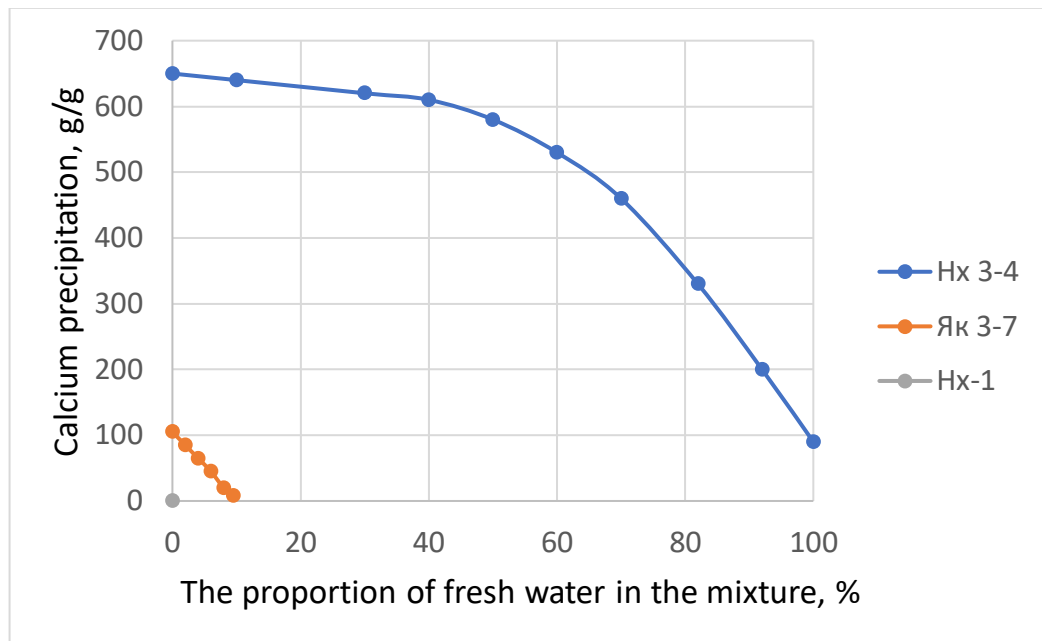
Picture 5 – Modeling of mixing of reservoir waters with manufactured and artesian in reservoir conditions
