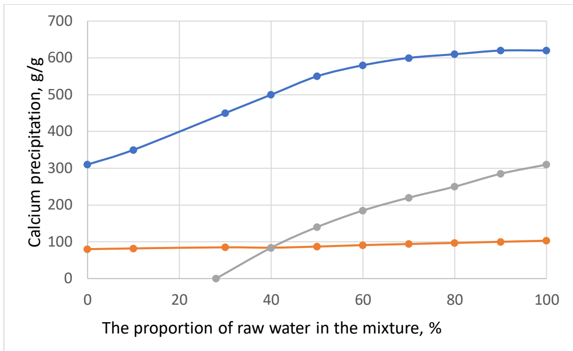
Picture 4 – Modeling of mixing of reservoir waters with manufactured and artesian in reservoir conditions
