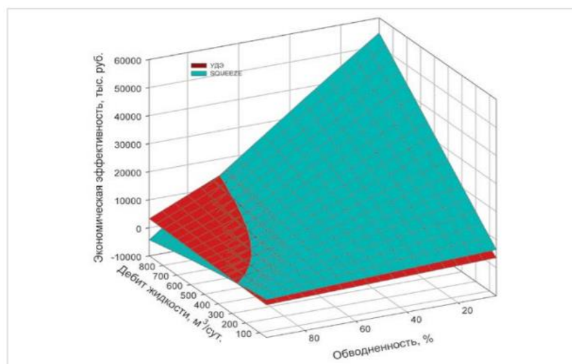
Picture 6 – Comparison of the economic efficiency of technologies for protecting wells from salt deposition by constant inhibition through a capillary (reagent dosing units) and by setting the inhibitor into the formation
