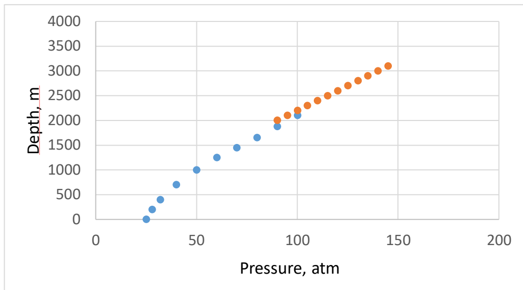
Picture 1 – Pressure changes along the borehole
