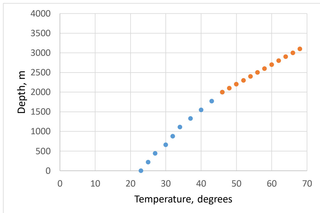
Picture 2– Temperature change along the borehole
