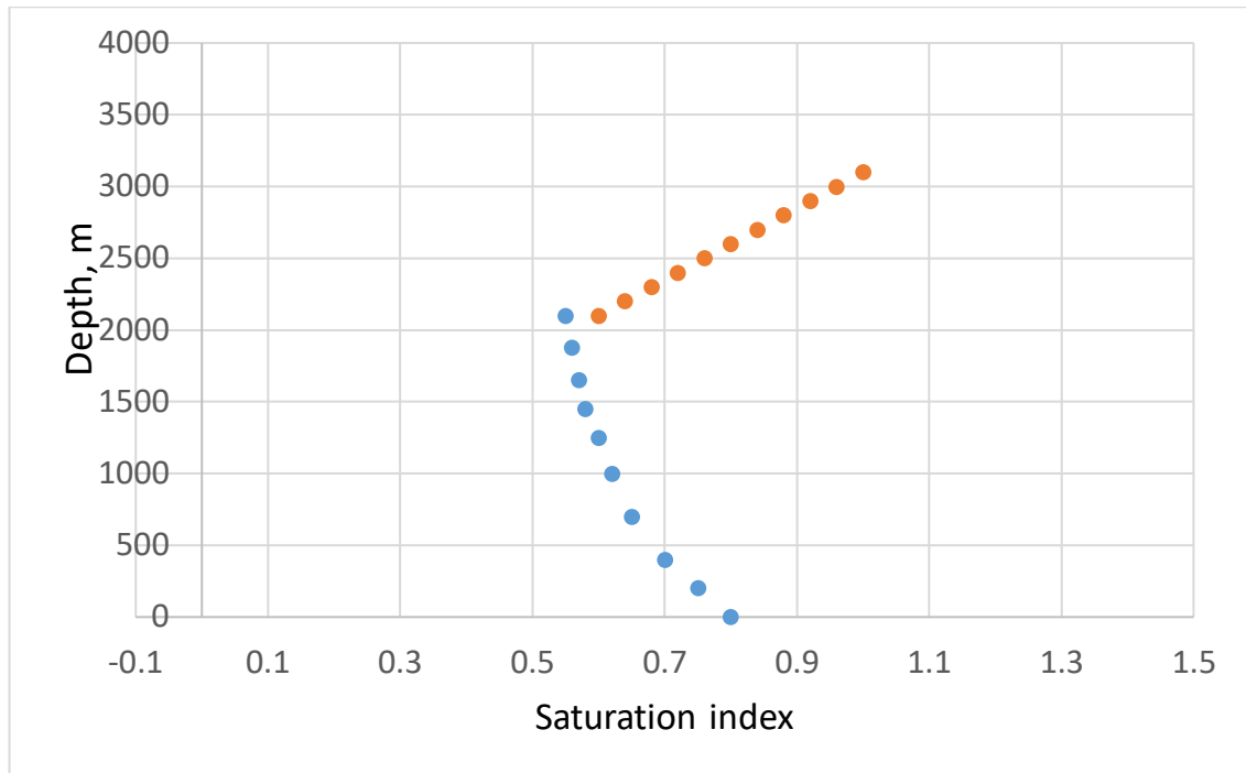
Picture 3 – Changes in the saturation index along the borehole
