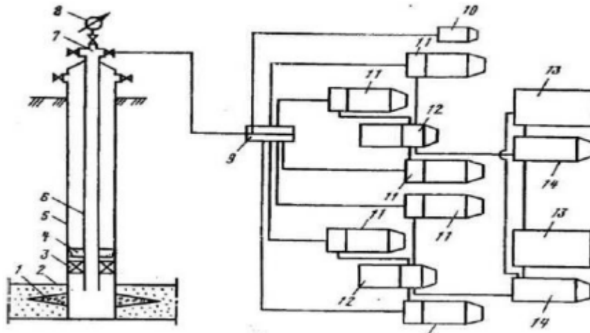
Figure 1 - Technological scheme of hydraulic fracturing: 1 - fracture; 2 - pay zone; 3 - packer; 4 - anchor; 5 - casing; 6 - tubing; 7 - wellhead fittings; 8 - manometer; 9 - manifold unit; 10 - process control and monitoring station; 11 - pumping units; 12 - sand mixers; 13 - tanks with process liquids; 14 - pump units
