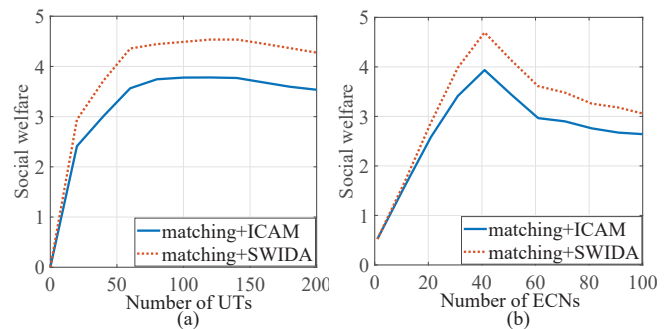
Fig. 5. Social welfare vs. (a) different numbers of UTs with M = 60 ECNs and (b) different numbers of ECNs with N = 40 UTs.
