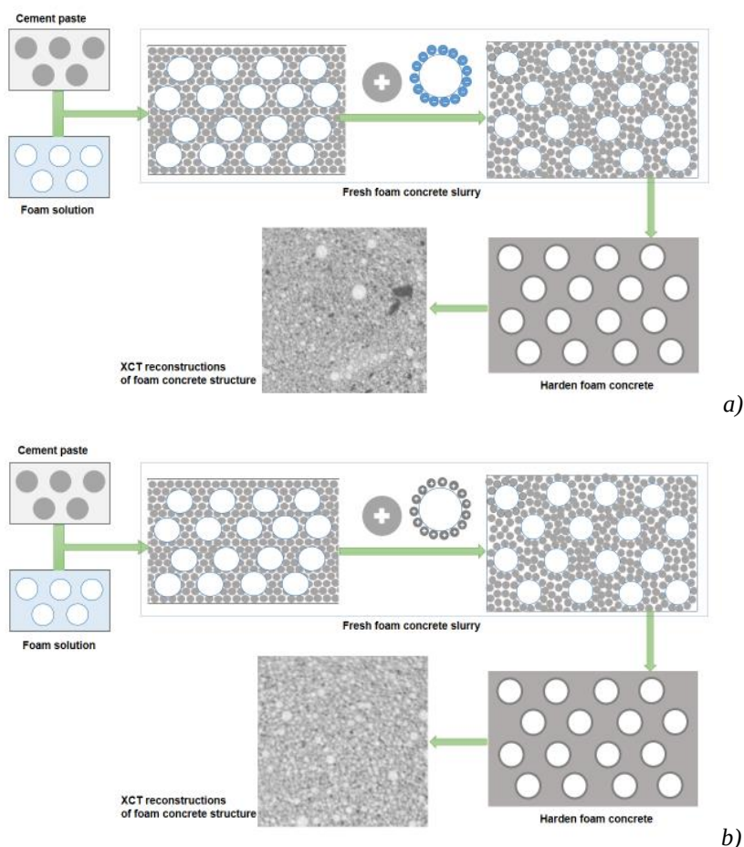
Fig. 1. The formation of the structure of non-autoclaved foam concrete: foam concrete (a), foam concrete with TMT600 additive (b)
