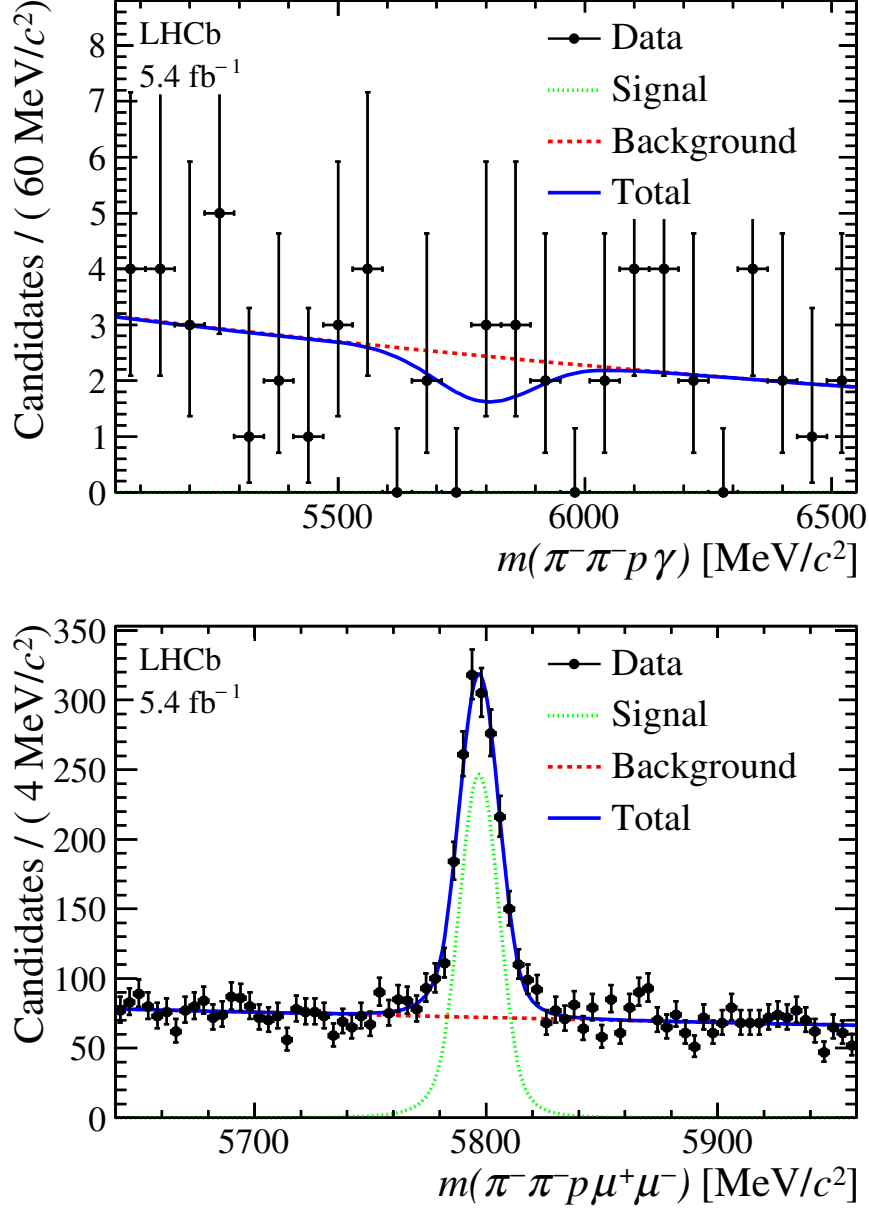
Figure 4. Distribution of (top) mass m(\pi^-\pi^-p\gamma) for selected \Xi^-\gamma ( \Xi^- \rightarrow \Lambda\pi^- ) and (bottom) m(\pi^-\pi^-p\mu^+\mu^-) for selected \Xi^-J/\psi ( J/\psi \rightarrow \mu^+\mu^- ) candidates. The projections of the simultaneous fit are overlaid.
