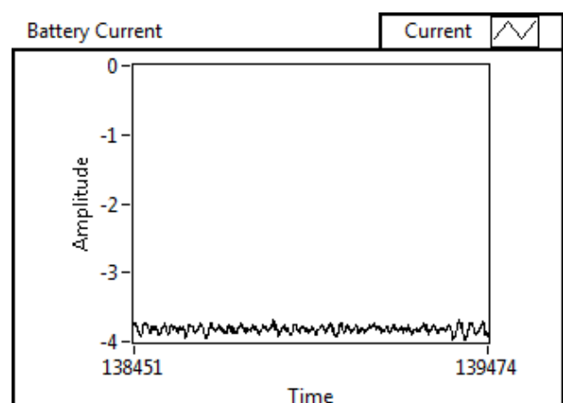
Fig. 11. Battery current
