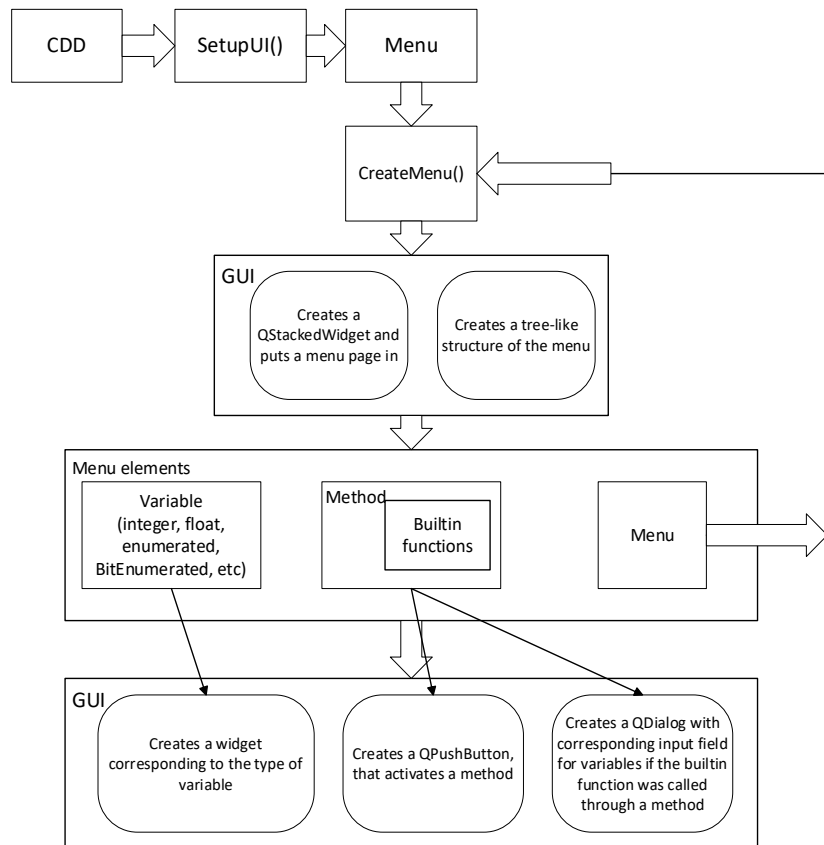
Fig. 1. A diagram of GUI creation in Colibri Software
