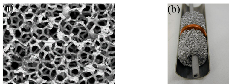
Figure 5. Aluminum foam (a) and metal hydride reactor with aluminum foam (b) [76].
