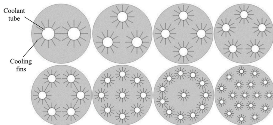
Figure 13. Cross-sectional configurations of the reactors with finned 2-, 3-, 4-, 5-, 6-, 9-, 12- and 18-pass heat exchangers, proposed by Keith M. D. et al. [110].
