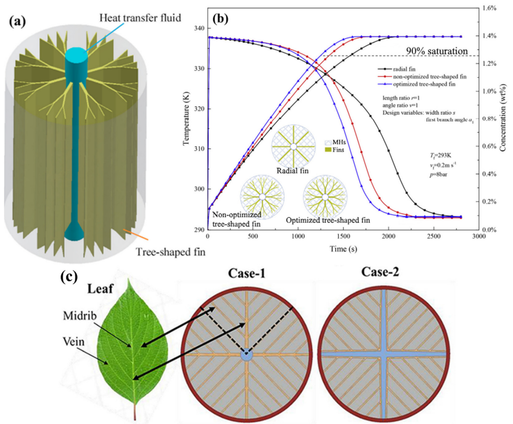
Figure 27. Heat exchanger with tree-shaped fins, proposed by Bai et al. (a) [168], comparison of the average bed temperature of tree-shaped fin heat exchanger with longitudinally finned heat exchanger (b) and bio-inspired heat exchangers designs, proposed by Krishna K. V. et al. (c) [169].
