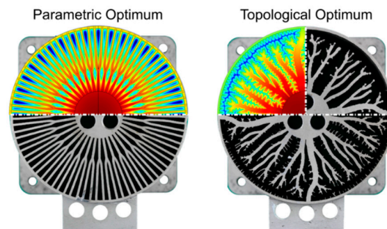
Figure 39. Heat sink designs: (left) with tree-shaped fins; (right) bio-inspired complex fins [217].
