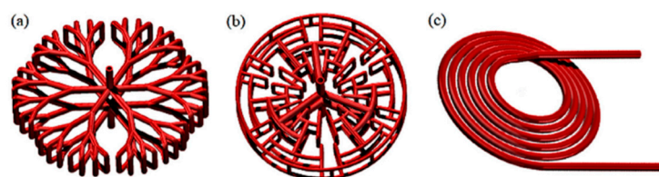
Figure 38. Fractal-tree-like heat sink designs: (a) Y-type; (b) H-type; and (c) traditional helical tube [216].
