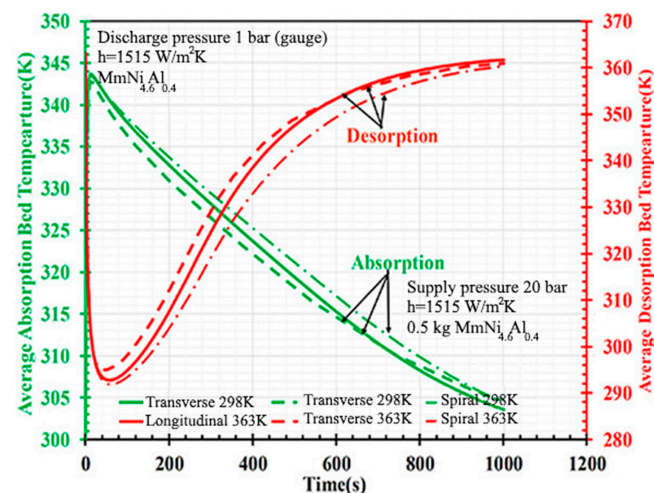
Figure 24. Average bed temperature for three configurations of heat exchanger, proposed by Parida A. and Muthukumar P. [164].
