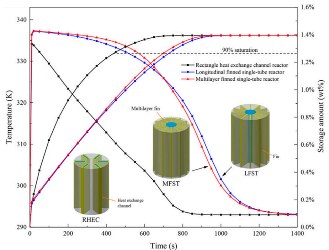
Figure 29. Influence of design on average bed concentration and temperature [173].
