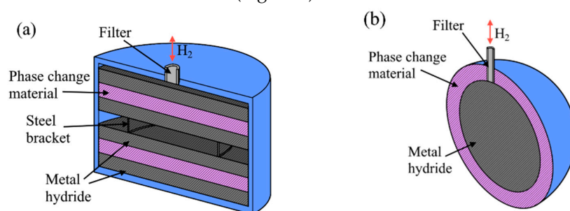
Figure 3. Different reactor shapes: (a) disk-shaped reactor and (b) spherical-shaped reactor.
