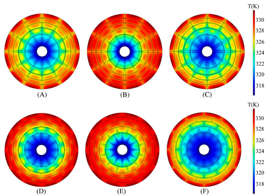
Figure 26. Temperature distribution of reactors with different multilayer heat exchanger configurations at 1000 s. (A) Aligned straight fin arrangement; (B) aligned fan-shaped fin arrangement; (C) aligned quadratic curve-shaped fin arrangement; (D) staggered straight fin arrangement; (E) staggered fan-shaped fin arrangement; (F) staggered quadratic curve-shaped fin arrangement [167].
