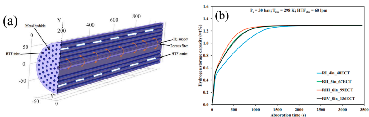
Figure 11. Metal hydride reactor with 99 embedded straight tubes, proposed by Raju N.N. et al. (a) [135], and effect of reactor geometry on variation of hydrogen storage capacity (in—diameter in inches; ECT—embedded cooling tubes; HTF—heat transfer fluid) (b).
