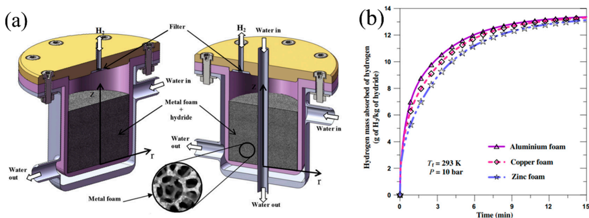
Figure 6. Metal hydride reactor with metal foam (a) and effect of base material on the storage time (b) [84].
