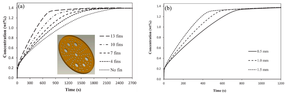
Figure 19. Effect of number of fins (a) and fin thickness (b) on average bed concentration [133].
