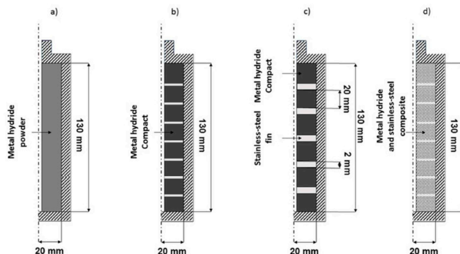
Figure 16. Schematic diagram of the different metal hydride bed configurations: (a) full Ti-Mn alloy powder bed (1st configuration), (b) Ti-Mn alloy compacts (2nd configuration), (c) alternating stainless steel fins and Ti-Mn alloy compacts (3rd configuration) and (d) a compact based on mixture of stainless steel and metal hydride powders (4th configuration) [152].
