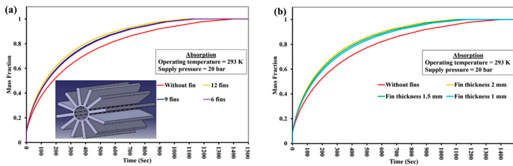
Figure 23. Influence of fin number (a) and fin thickness (b) on hydrogen absorption rate. Inset: finned tube heat exchanger, proposed by Gupta S. and Sharma V. K. [163].
