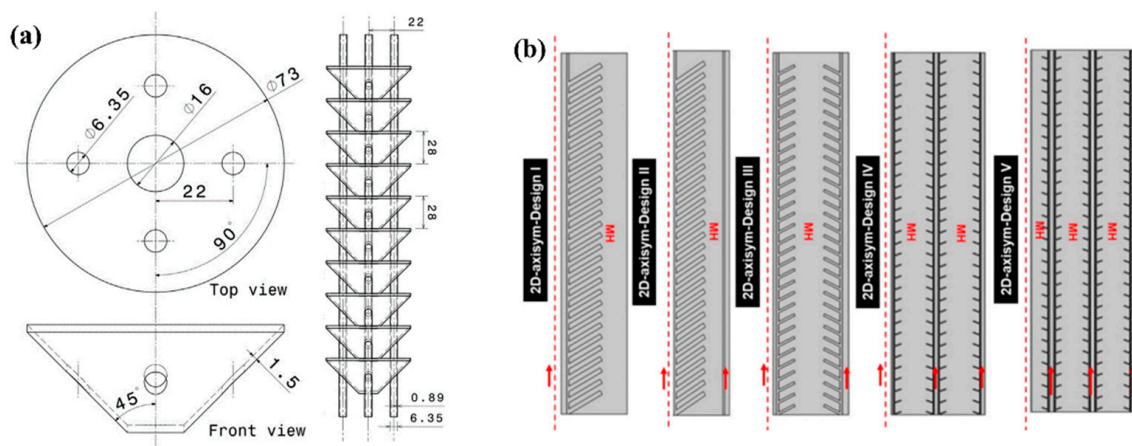
Figure 20. Heat exchanger with conical fins, proposed by Chandra et al. (a) [159] and various configuration of metal hydride reactors with conical fins, proposed by Ayub I. et al. (b) [160].
