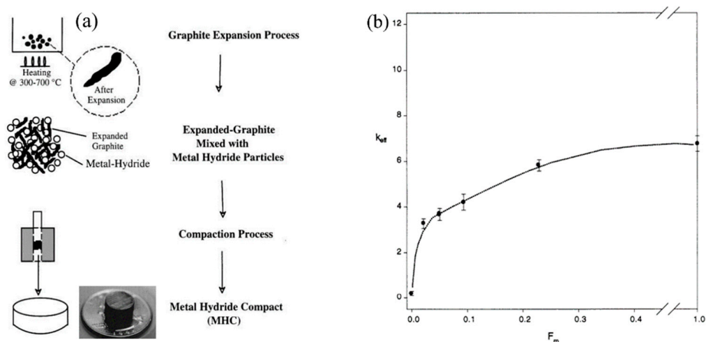
Figure 4. A schematic of recompressed expanded graphite technique (a) and measured effective thermal conductivity of metal hydride compacts versus mass fraction of graphite (b) [64].
