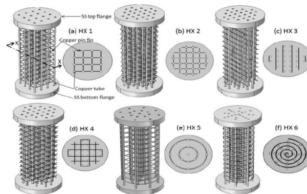
Figure 36. Different complex heat exchanger designs, proposed by Keshari V. and Maiya M. P. [213].
