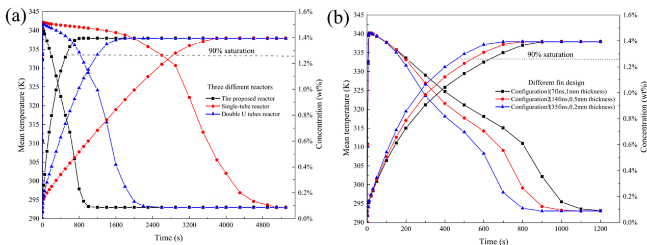
Figure 10. Effect of different reactors (a) and fin configuration (b) on the bed temperature and hydrogen concentration [111].
