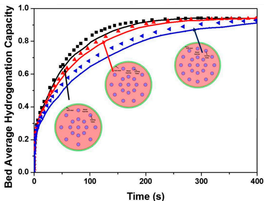
Figure 14. The comparison of the average hydrogenation capacity for metal hydride reactor with 12 cooling tubes (black), 16 cooling tubes (red) and cooling 20 tubes (blue). The solid line indicates the results obtained by Gkanas E. I. et al. [140], while the dotted line indicates the results obtained by Muthukumar P. et al. [139].
