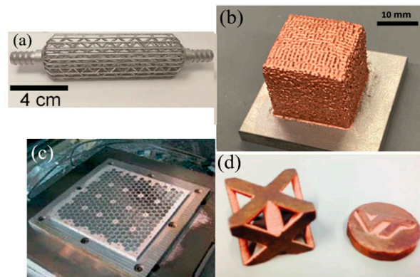
Figure 34. Metal parts obtained using different printing technologies: (a) heat exchanger, fabricated from AlSi10Mg using DMLS [207]; (b) 20 mm × 20 mm × 20 mm copper cube with density of 94.1% built using blue laser [200]; (c) aluminum honeycomb structure, manufactured by SL method [210]; (d) complex-shaped copper made via binder jetting [205].
