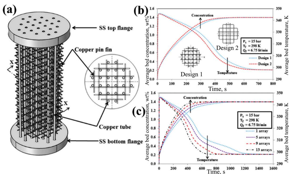
Figure 28. Heat exchanger with pin fins, proposed by Keshari V. and Maiya M. P. (a) [160], and influence of design (b) and number of pin fin arrays for design 1 (c) on average bed concentration and temperature.
