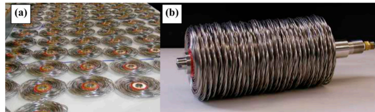
Figure 30. Heat exchanger for metal hydride compressor, proposed by Lototskyy M. V. (a); hydride tube ring manifolds; (b) the manifolds stacked into hydride heat exchanger [48].
