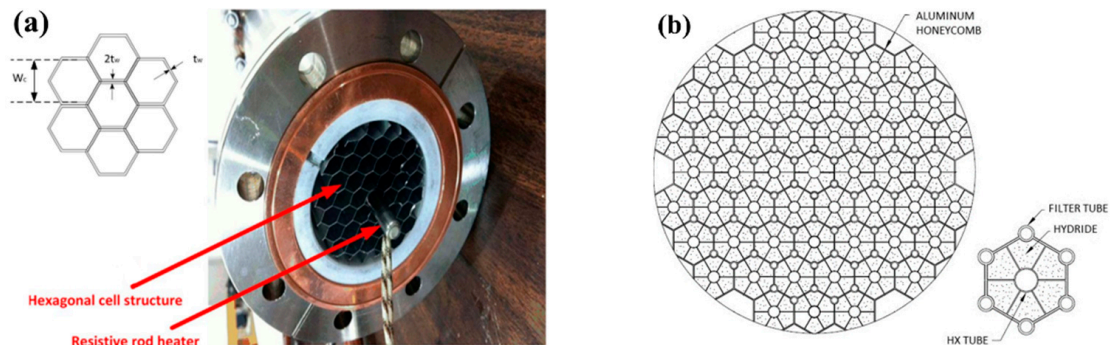
Figure 25. Honeycomb cell structure for metal hydride reactor, proposed by Corgnale C. et al. (a) [165] and George M. and Mohan G. (b) [166].
