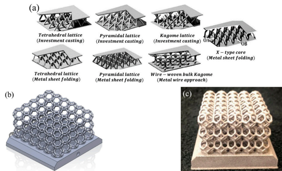
Figure 35. 3D-printed cell structures: (a) metal sandwich panels with different lattice structures [210]; (b) lattice-structured heat sink design; and (c) heat sink manufactured using additive manufacturing [211].
