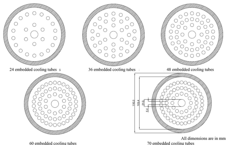
Figure 12. Reactor configurations with embedded cooling tubes, proposed by Anbarasu S. et al. [137].
