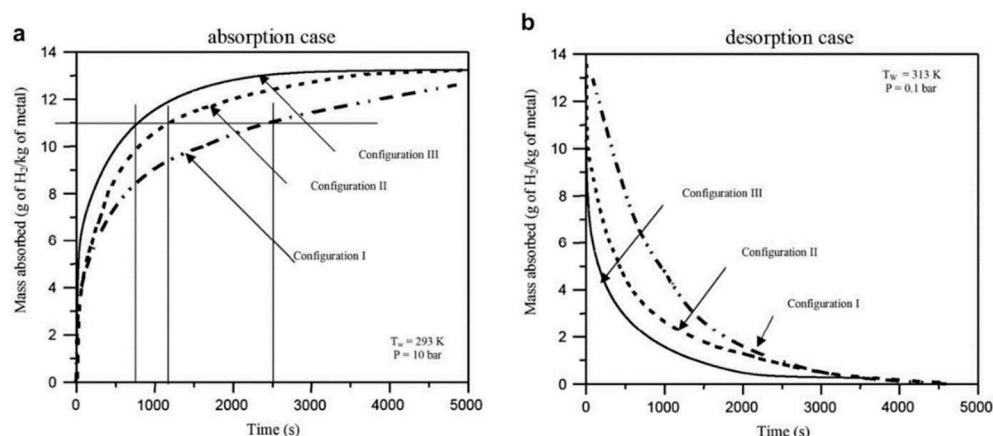
Figure 7. Time evolution of the hydrogen mass stored (a) and desorbed (b) in three different metal hydride reactor configurations [113].
