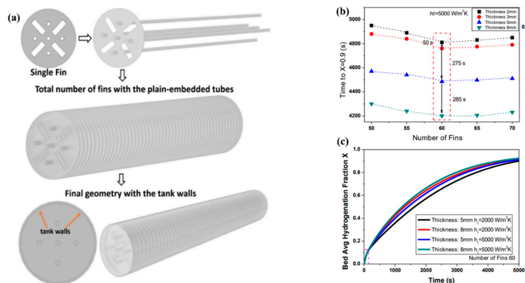
Figure 17. Heat exchanger design, proposed by Gkanas E. I. et al. (a) [154]; influence of number of fins on the time to attain 90% saturation with a dotted square area indicating the number of fins after which there is no improvement in reaction speed (b); and fin thickness on the average hydrogenation fraction (c).
