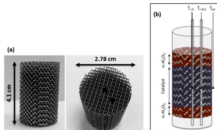
Figure 37. Conductive periodic open cellular structure: (a) manufactured heat exchanger; (b) qualitative scheme of the heat exchanger embedded into the Fischer–Tropsch fixed-bed reactor [215].
