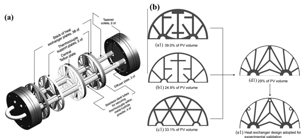
Figure 22. Heat exchanger (a) and fin geometry optimization (b) [94].
