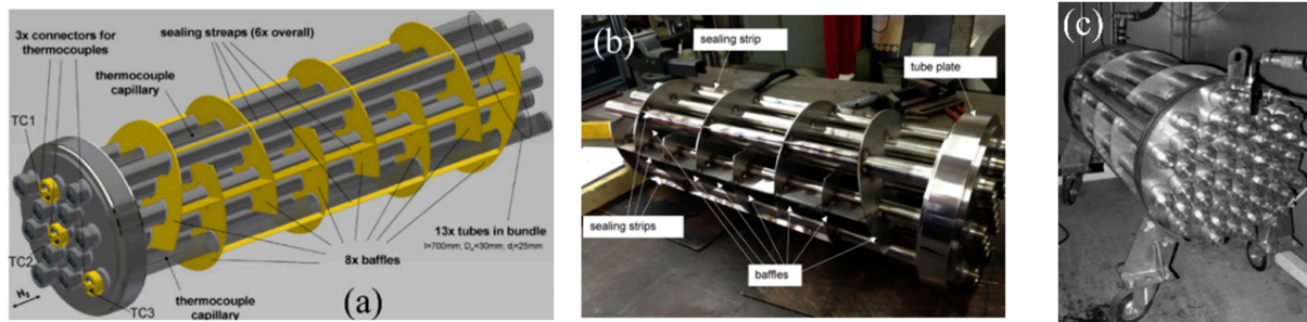
Figure 33. Large-scale hydrogen storage reactors: (a) tube bundle heat storage reactor model; (b) tube bundle metal hydride reactor [184]; (c) metal hydride storage system PX-1 [46].
