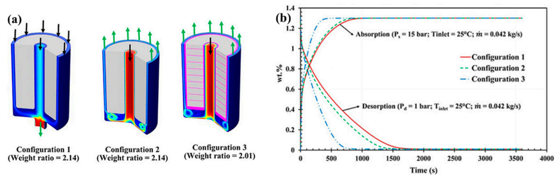
Figure 21. Three different configurations of annular metal hydride reactor (a) and hydrogen sorption/desorption rates for proposed configurations (b) [161]. The heat exchanger fins are highlighted in purple. The black arrow indicates the inlet of heat transfer fluid and the green arrow indicates the outlet of heat transfer fluid.
