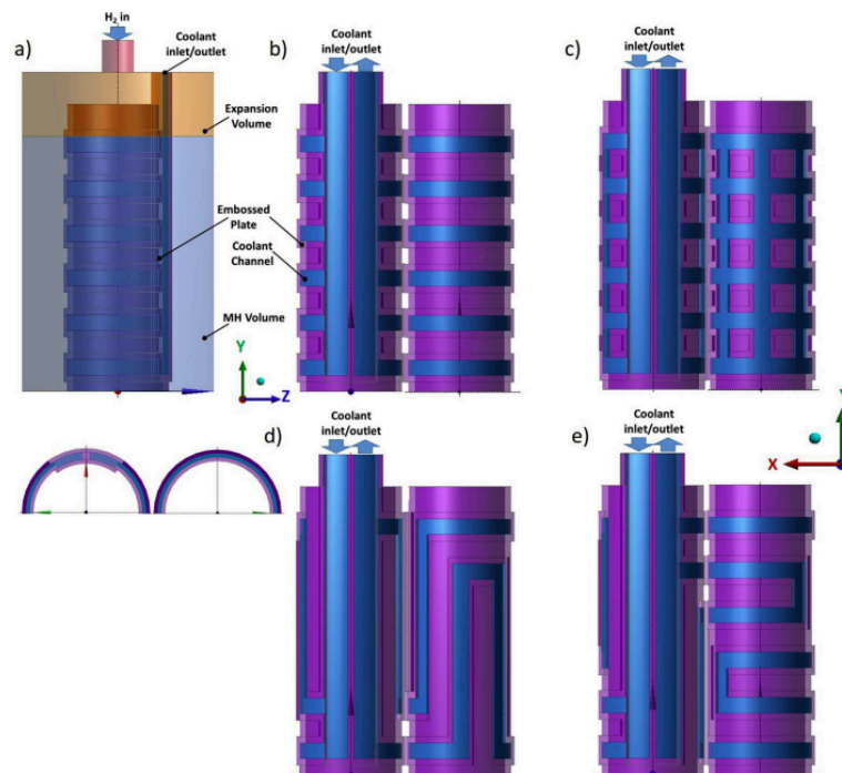
Figure 31. Configurations of the metal hydride storage systems with embossed plate heat exchanger, proposed by Lewis et al. [175]: (a) parallel flow-field embossed plate heat exchanger; (b) parallel-type configuration; (c) pin-type configuration; (d) vertical serpentine configuration; (e) horizontal serpentine configuration.
