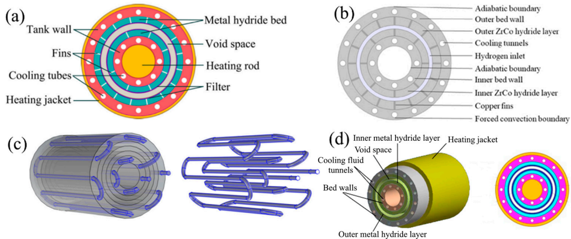
Figure 32. Annular reactors: (a) thin double-layered hydrogen ZrCo-based hydride bed, proposed by Zhang B. et al. [178]; (b) double-layered cylindrical ZrCo hydride bed, proposed by Li W. et al. [177]; (c) circular-shaped cooling pipe, proposed by Zhang B. et al. [178]; (d) thin double-layered annulus bed, proposed by Cui Y. et al. [176].
