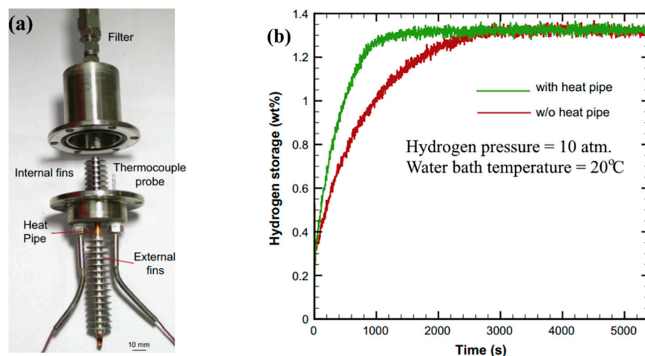
Figure 15. Prototype of the metal hydride reactor, proposed by Chung C. A. et al. (a) [151], and influence of heat exchanger on hydrogen sorption rate (b).
