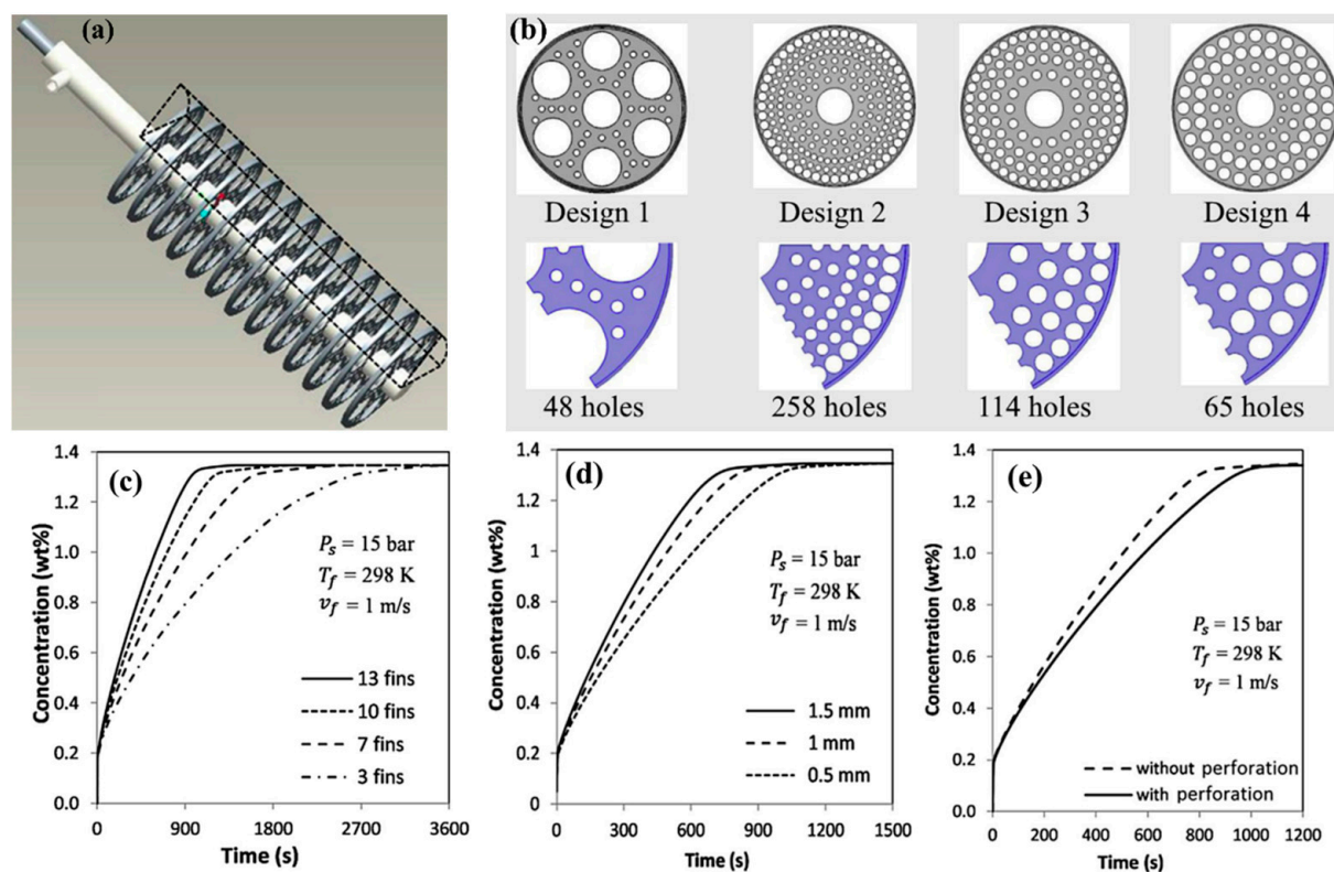
Figure 18. Heat exchanger (a), different designs of copper fins (b), proposed by Singh A. et al. [157], and effect of different fin number (c), thickness (d) and perforation (e).
