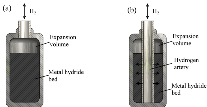
Figure 2. Different metal hydride reactor types: (a) chamber (tank) reactor; (b) tubular reactor.
