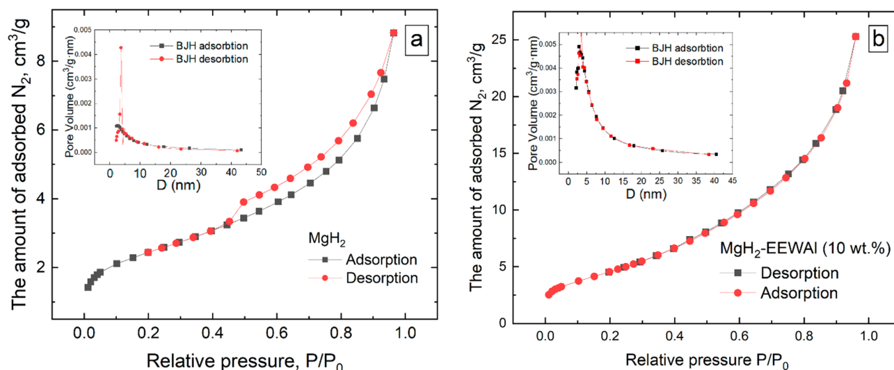
Figure 3. BET absorption and desorption curves at 77 K with pore size distribution (PSD) for \text{MgH}_2 (a) and \text{MgH}_2 -EEWAl (b) composite.
