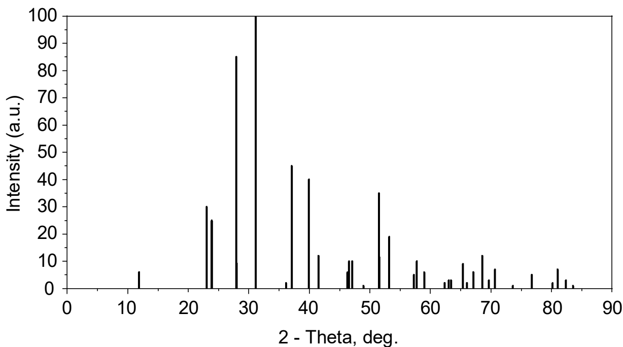
Figure 2. XRD analysis of a BaFBr single crystal sample.
