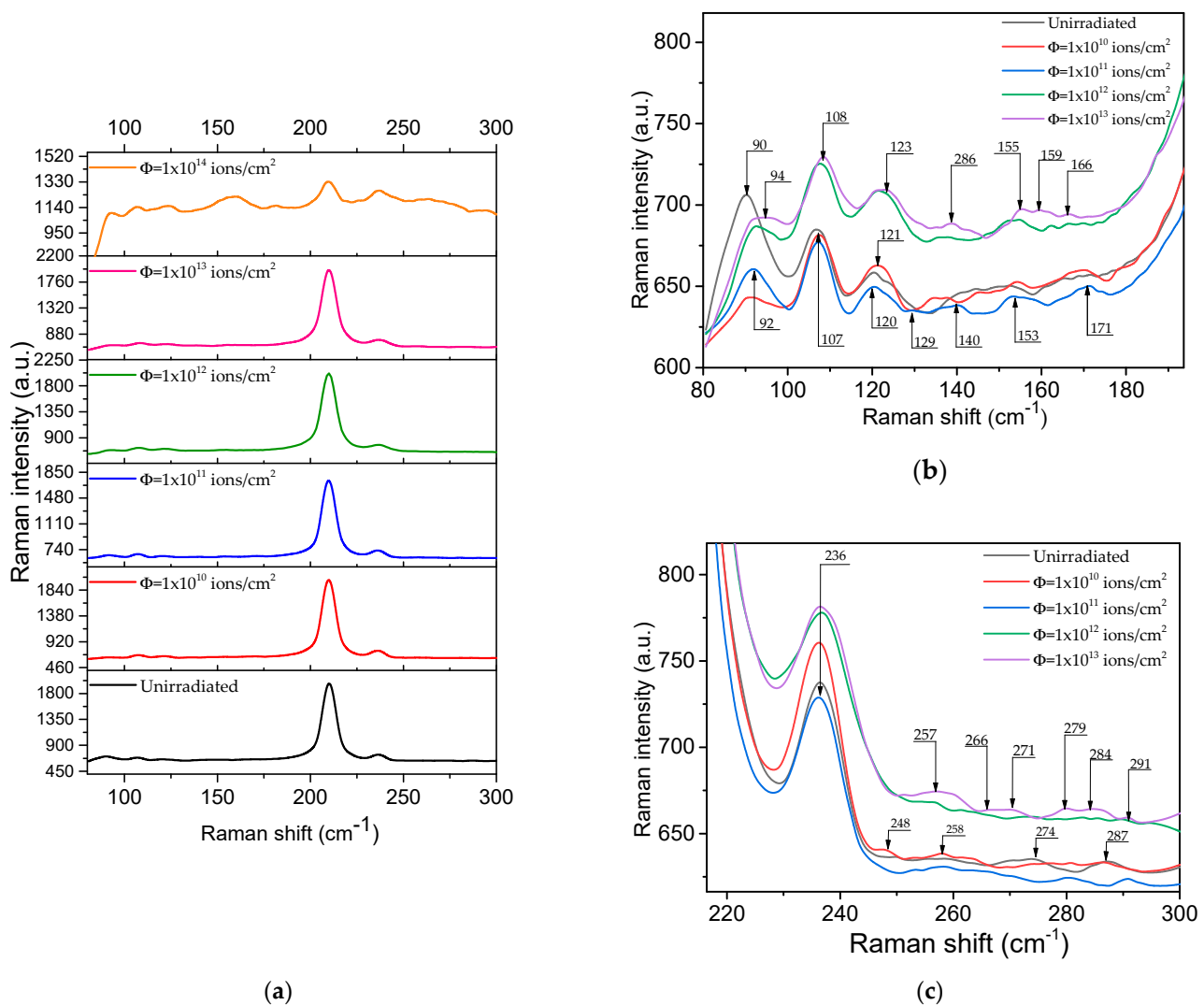
Figure 7. Raman spectra of BaFBr as a function of ion fluence, shown for different spectral ranges: 80–300 cm -1 (a), 80–195 cm -1 (b) and 210–300 cm -1 (c).
