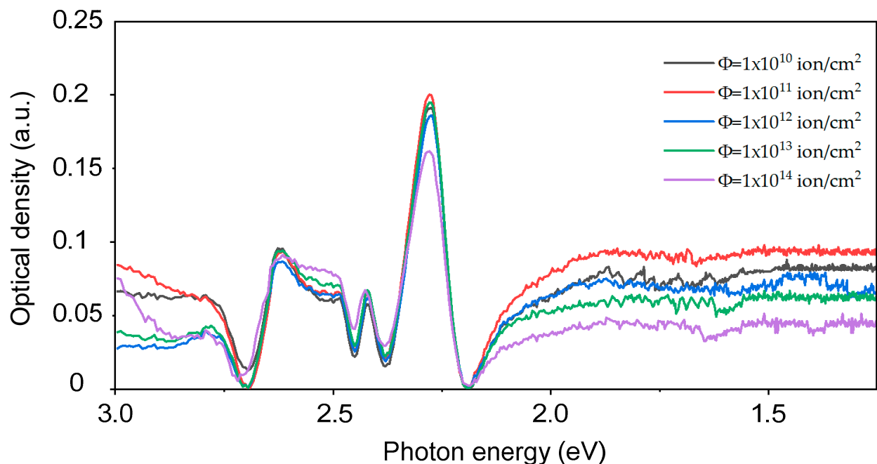
Figure 5. Absorption spectra of BaFBr irradiated with ions 147 MeV 84 Kr. Fluence range ( 1 \times 10^{10} ion/cm 2 – 1 \times 10^{14} ) ion/cm 2 .
