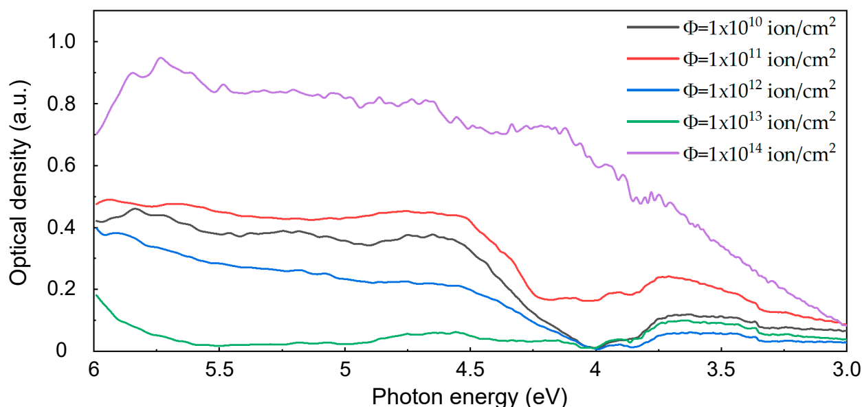
Figure 6. Absorption spectra of BaFBr irradiated with 147 MeV ^{84}\text{Kr} ions. Fluence range ( 1 \times 10^{10} – 1 \times 10^{14} ) \text{ion}/\text{cm}^2 .
