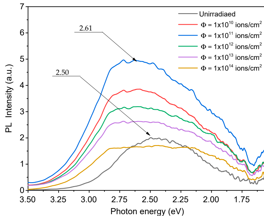
Figure 4. PL spectra of BaFBr crystals irradiated with 147 MeV ^{84}\text{Kr} ions at 300 K to fluences 1 \times 10^{10} – 1 \times 10^{14} ion/cm ^2 . Excitation wavelength \lambda = 280 nm.
