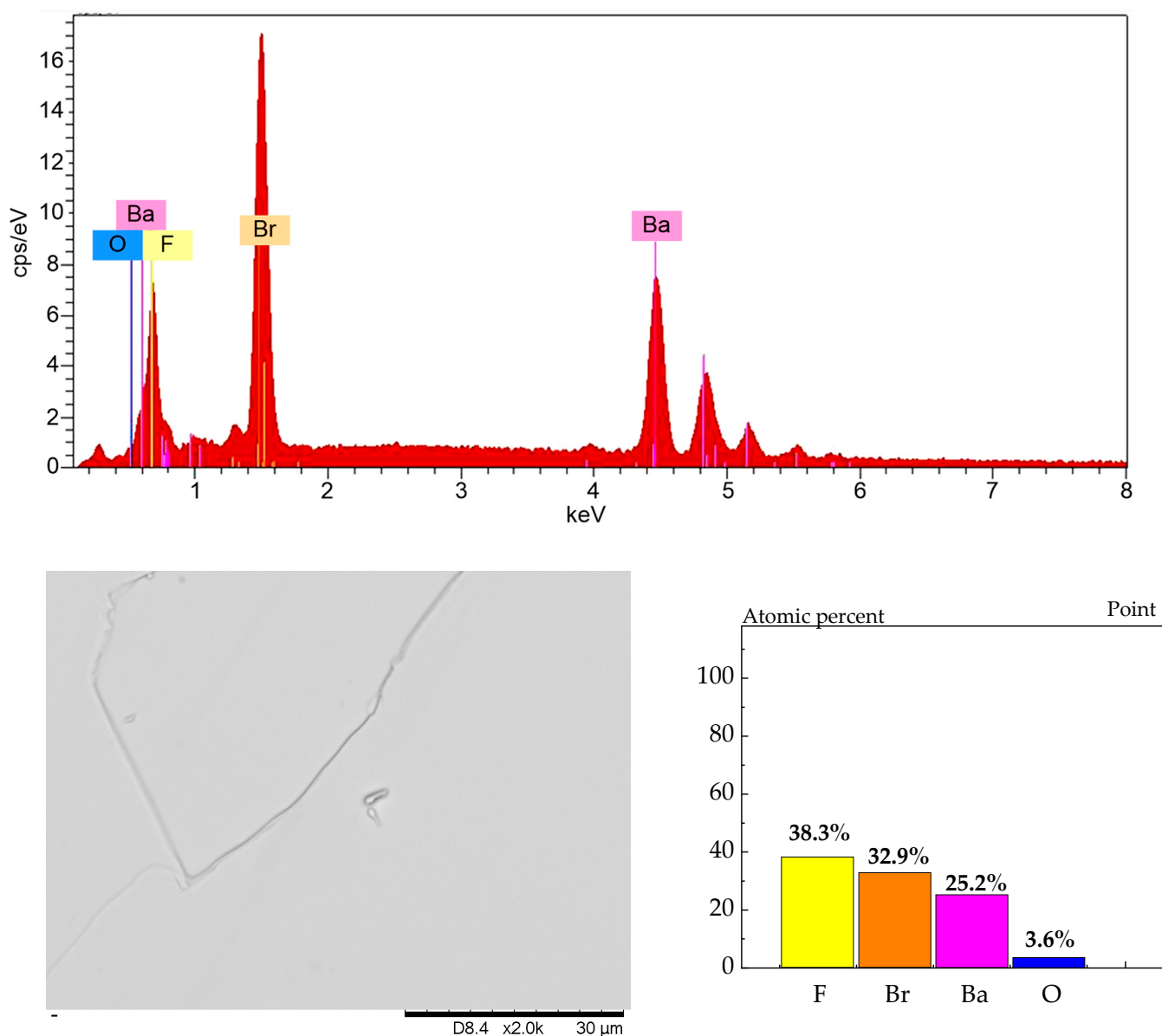
Figure 1. Elemental analysis (EDX) of BaFBr crystals. The lower left corner shows an example of the surface of one of the crystals.
