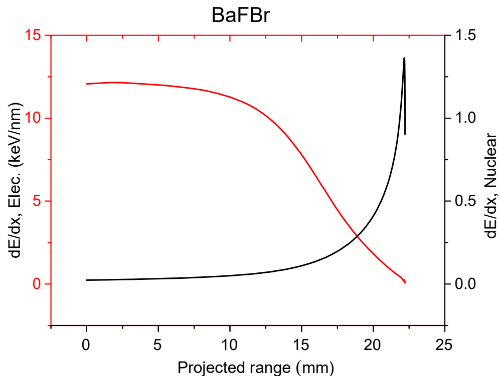
Figure 3. Electronic energy loss (red) and nuclear energy loss (black) of BaFBr crystals irradiated with 147 MeV ^{84}\text{Kr} ions.
