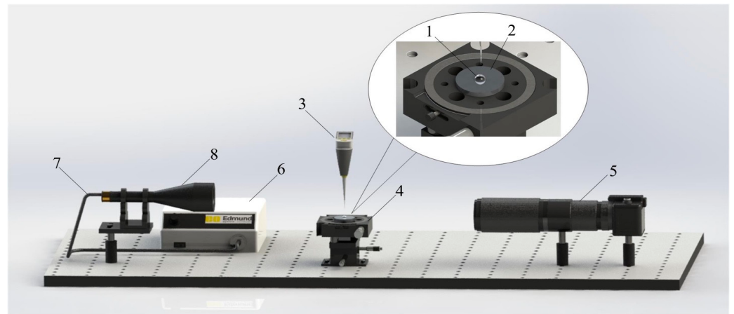
Figure 1. Experimental setup for measuring the static contact angles formed by liquid droplets and solid surfaces (AMG-6, PTFE): 1—liquid droplet; 2—AMG-6 or PTFE discs; 3—electronic dispenser; 4—goniometer; 5—camera; 6—light source; 7—fiber optic cable; 8—telecentric tube.
