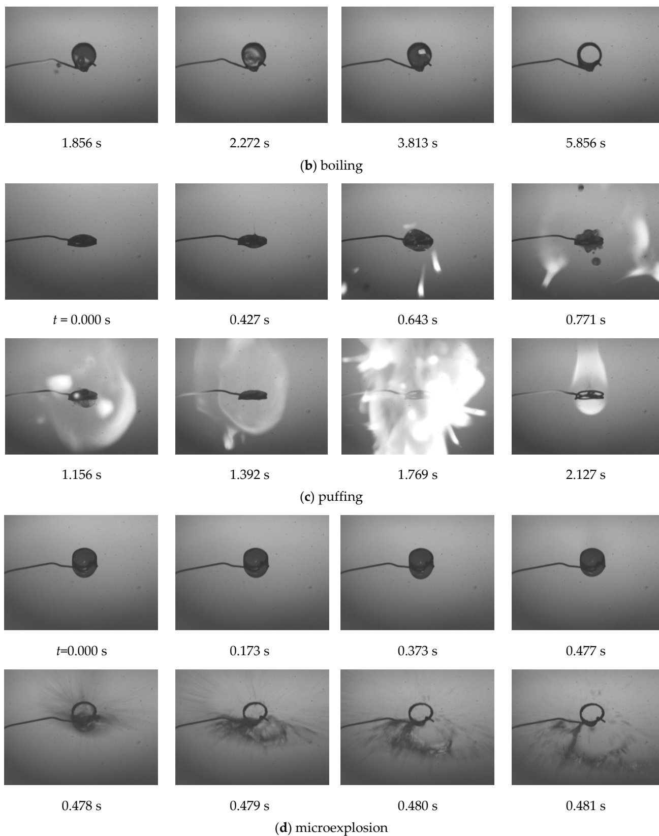
Figure 3. Typical frames of videograms illustrating the four mechanisms of physical and chemical processes during the high-temperature heating of binary liquids: (a) evaporation (acetone–95% ethyl alcohol); (b) boiling (water–acetone); (c) puffing (ethylene glycol–compressor oil); (d) microexplosion (monoethylamine–diiodomethane).
