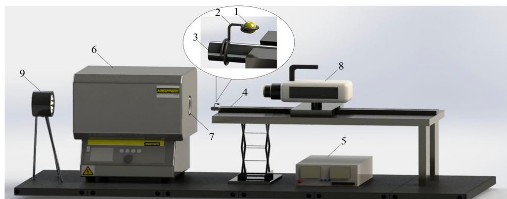
Figure 2. Experimental setup: 1—liquid droplet; 2—holder; 3—steel tube; 4—coordinate mechanism; 5—control unit of the coordinate mechanism; 6—muffle furnace; 7—ceramic tube; 8—high-speed video camera; 9—LED lamp.
