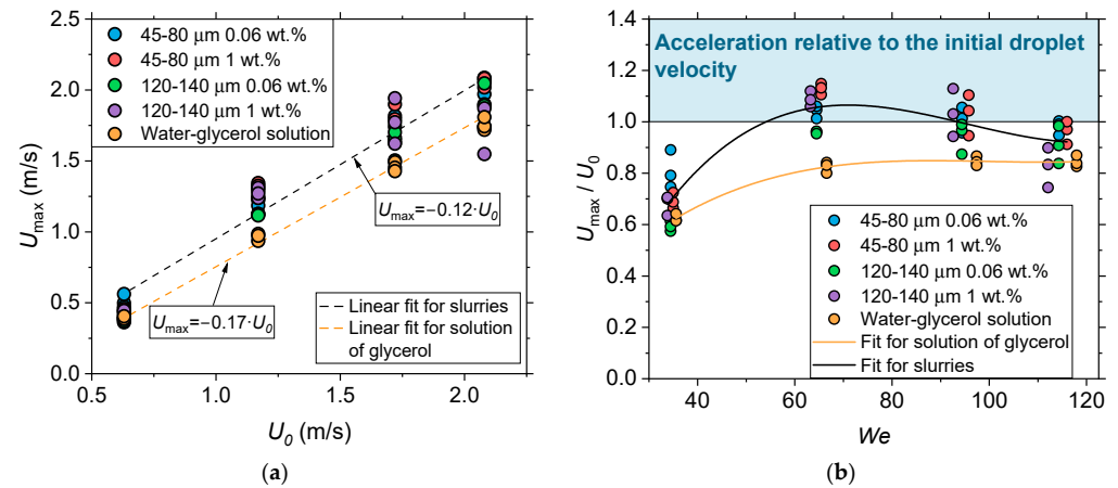
Figure 7. Maximum absolute velocities of internal flows in a drop U_{\max} as a function of the initial velocity of the drop before impact U_0 (a), parameter U_{\max}/U_0 as a function of We (b).
