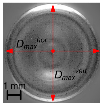
Figure 3. Illustration of the approach to analyzing the maximum drop spreading diameter D_{\max} in shadow photography of the collision process.
