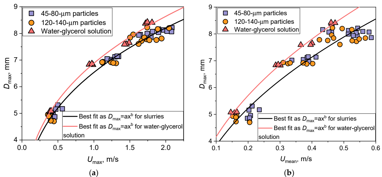
Figure 9. Effect of U_{\max} (a) and U_{\text{mean}} (b) on the maximum spreading diameter at different grinding finenesses of coal particles.
