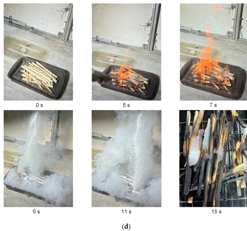
Figure 15. Snapshots of wood fire ( m_w \approx 70 g) being suppressed using carbon dioxide hydrate powder: (a) m_g \approx 7 g; (b) m_g \approx 15 g; (c) m_g \approx 30 g; (d) m_g \approx 100 g.
