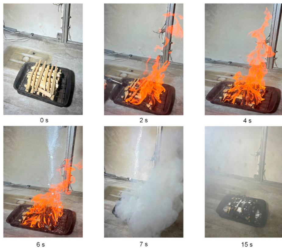
Figure 16. Snapshots of the suppression of a model wood crib fire with several tiers using carbon dioxide hydrate powder: m_g \approx 80 g.
