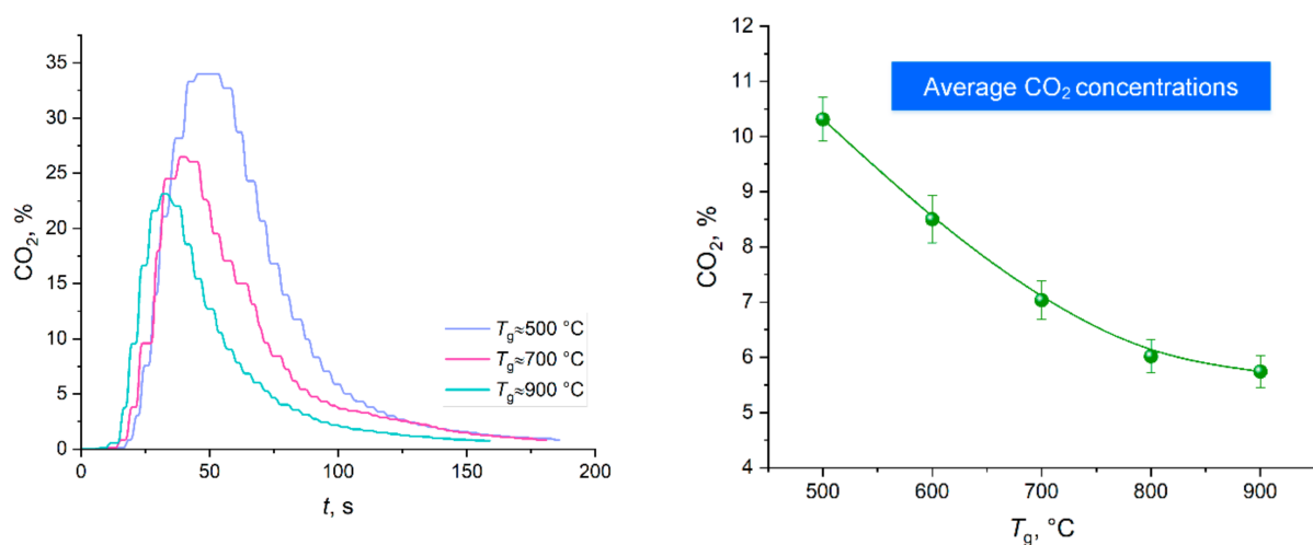
Figure 8. \text{CO}_2 concentrations from the thermal decomposition of carbon dioxide hydrate tablet at varying temperatures in the muffle furnace: changes in the concentration over time (on the left); average concentrations (on the right).
