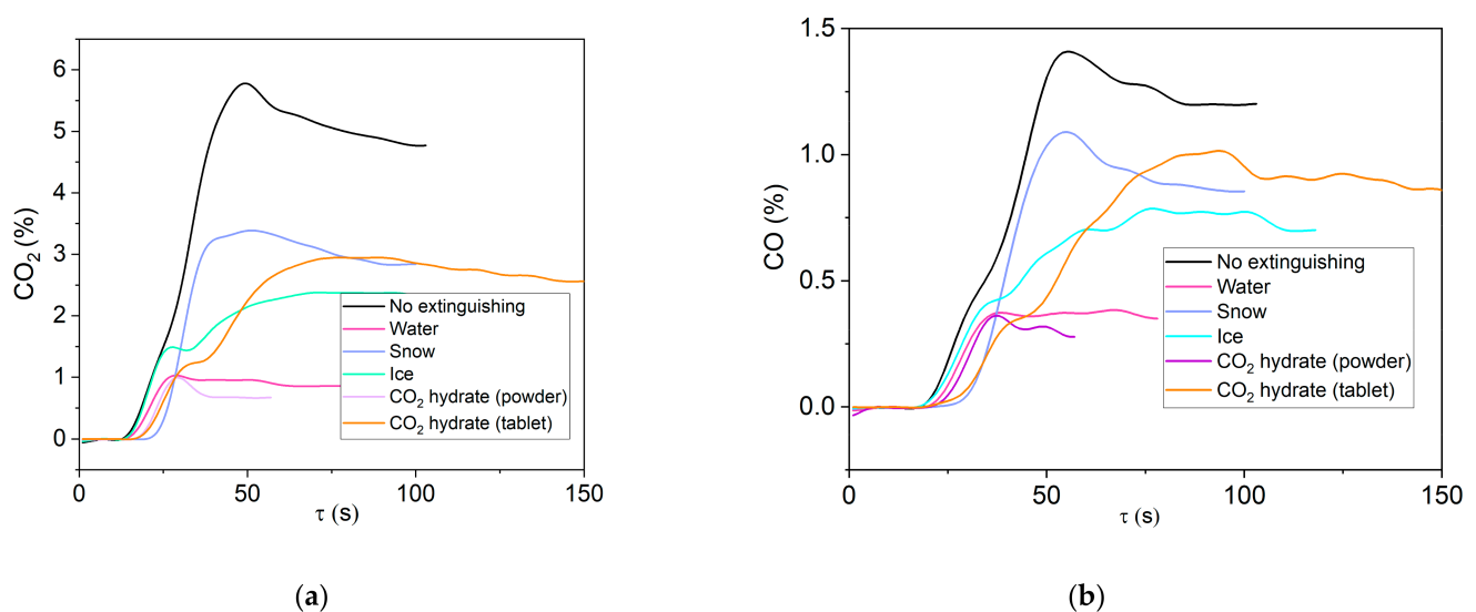
Figure 10. Concentrations of \text{CO}_2 (a) and CO (b) emitted during wood fire suppression.
