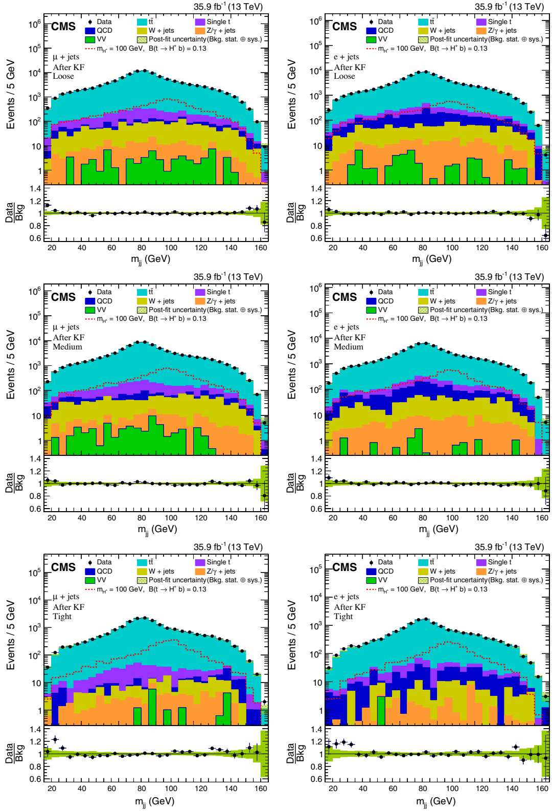
FIG. 3. Distributions of m_{jj} after a background-only fit to the data, in the exclusive charm tagging categories for the muon + jets (left column) and electron + jets (right column) channels. The upper row shows the exclusive loose category, the middle row shows the exclusive medium category, and the lower row shows the exclusive tight category. The expected signal significance (prior to the fit) can be observed to vary across the different categories. The uncertainty band (showing the absolute uncertainty in the upper panels and the relative uncertainty in the lower panels) includes both statistical and systematic components after the background-only fit. The signal distributions are scaled by twice the maximum observed upper limit on \mathcal{B}(t \rightarrow H^+ b) obtained at 8 TeV [23].
