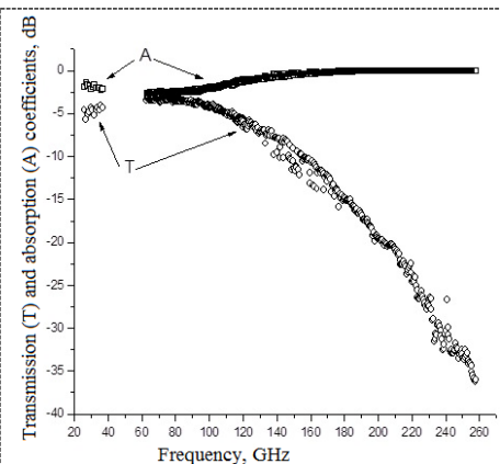
Figure 3. Parameters of the electromagnetic response of the sample synthesized from the foam glass-ceramic material.
