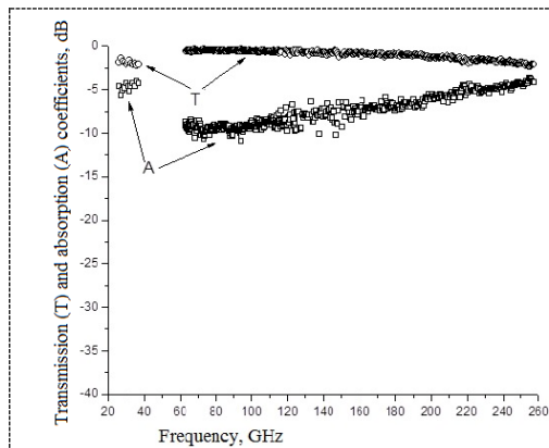
Figure 2. Parameters of the electromagnetic response of the sample synthesized from commercially available glass cullet.
